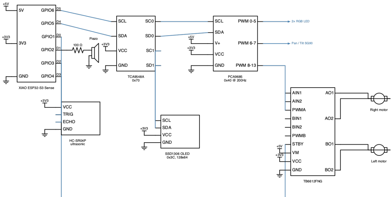
Figure 1: Full wiring schematic. Source: docs/schematics/circuits/robocar_unified.py.
