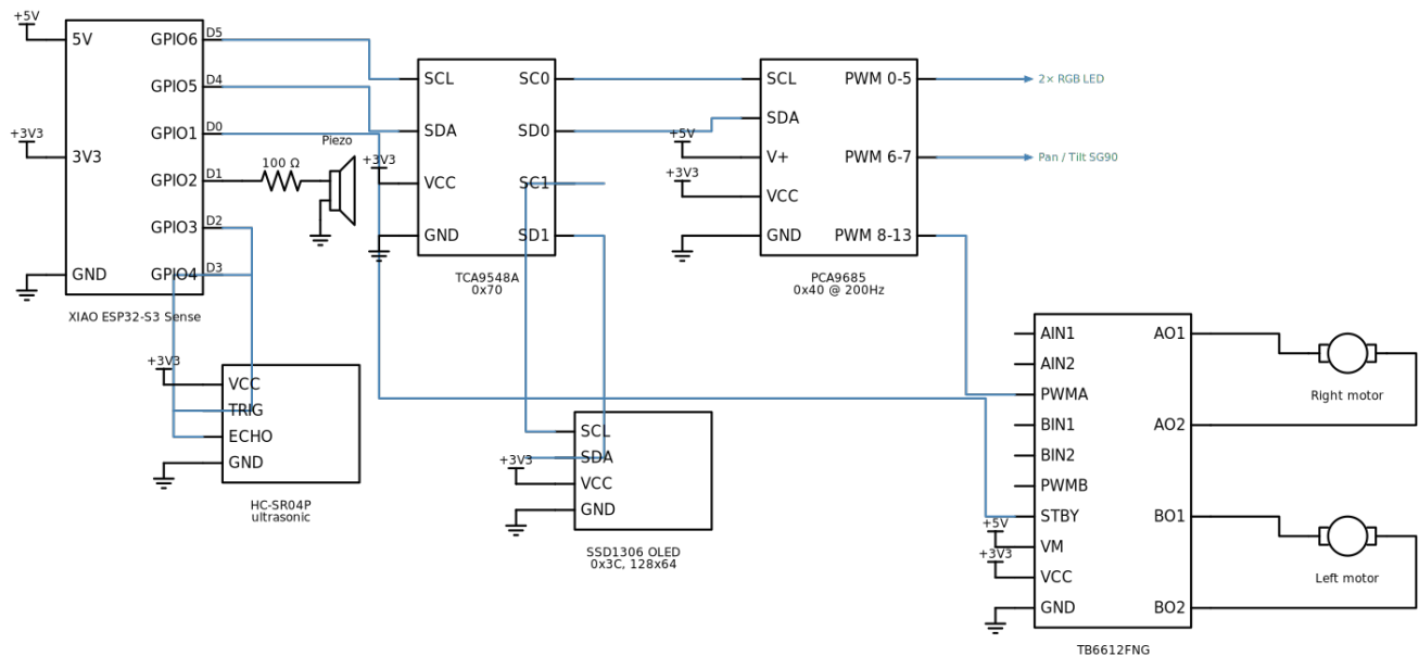
Figure 1: Full wiring schematic. Source: docs/schematics/circuits/robocar_unified.py.
