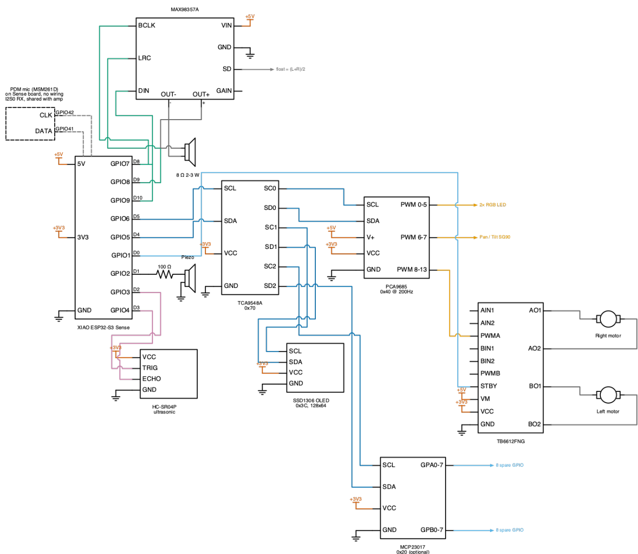
Figure 1: Full wiring schematic. Source: docs/schematics/circuits/robocar_unified.py.
