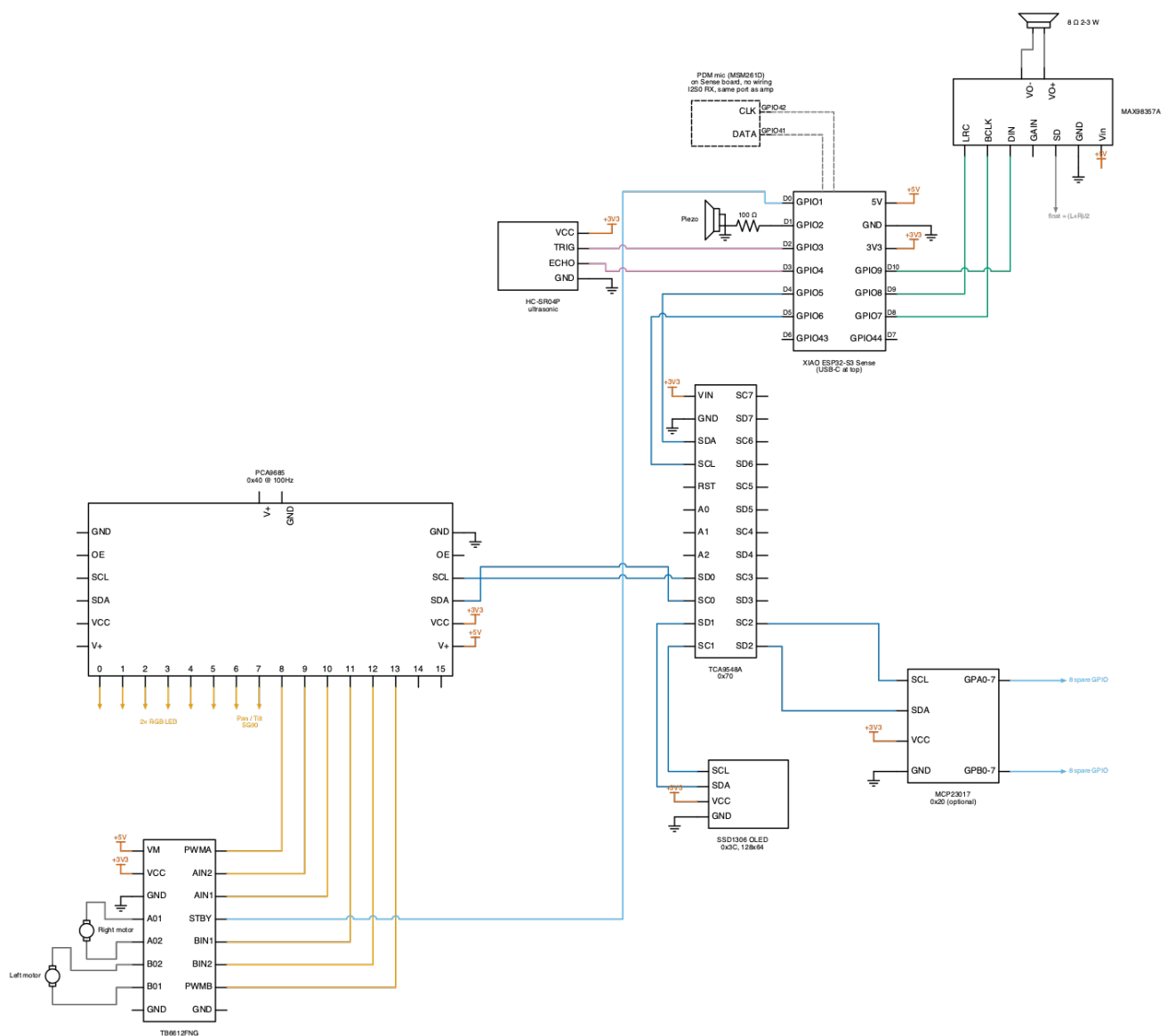
Figure 1: Full wiring schematic. Source: docs/schematics/circuits/robocar_unified.py.
