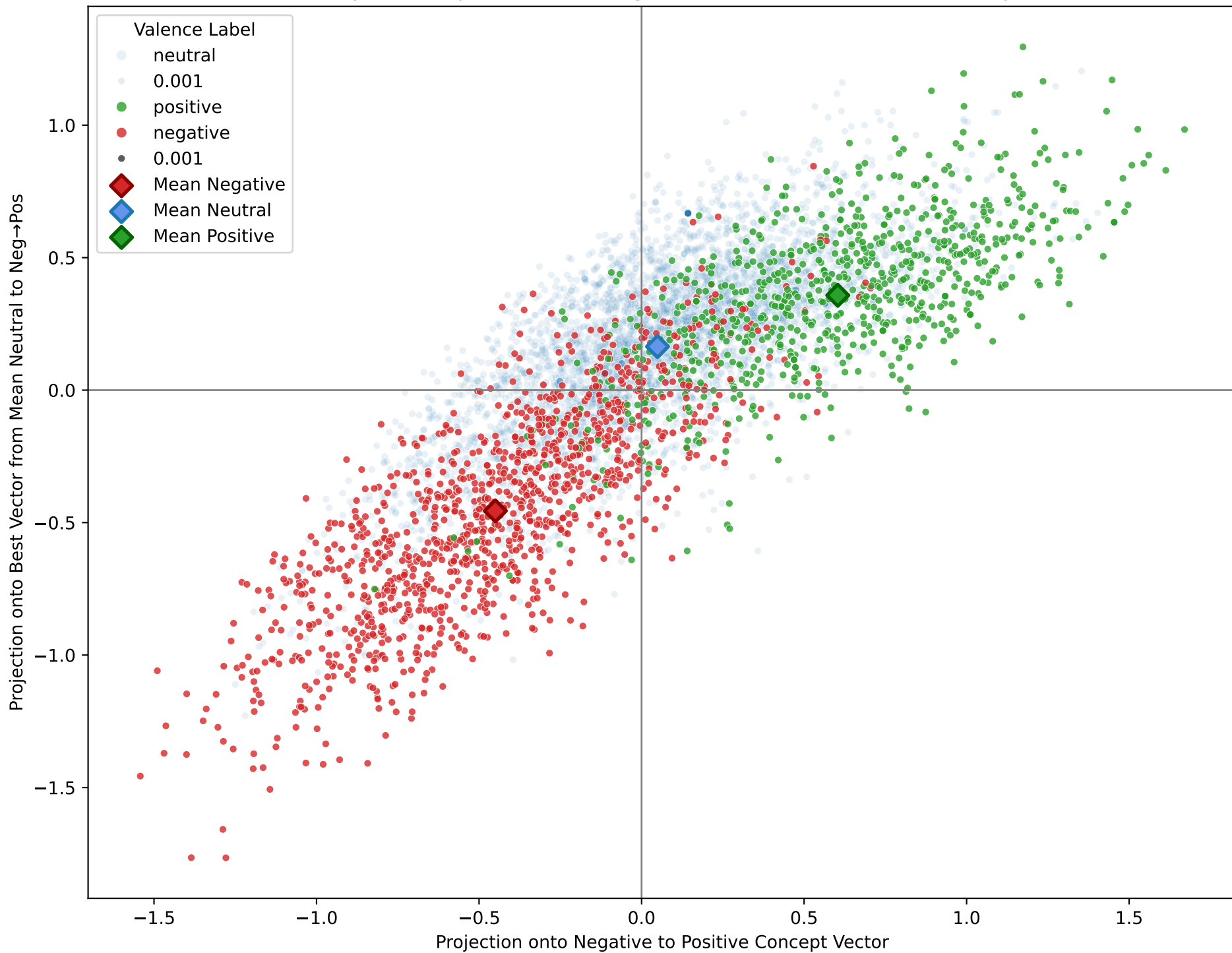
Scatterplot of Projections onto Neg→Pos vs. Best Vector (Fiction4 Corpus)
