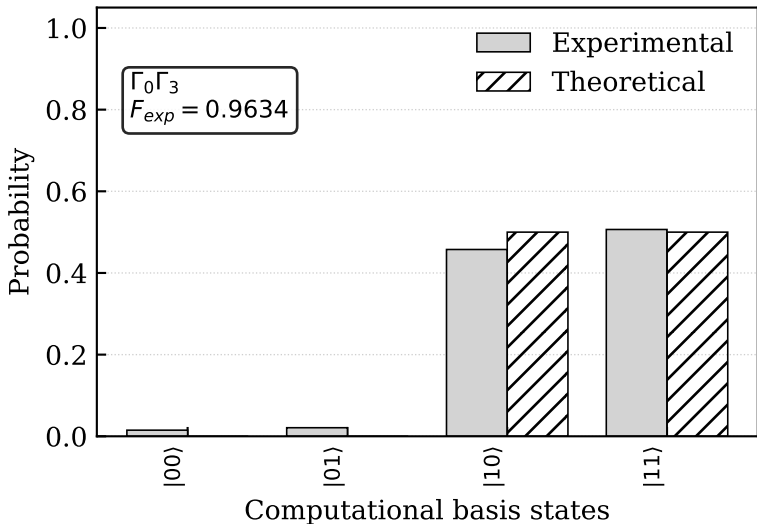
Histogram for algorithm 2
