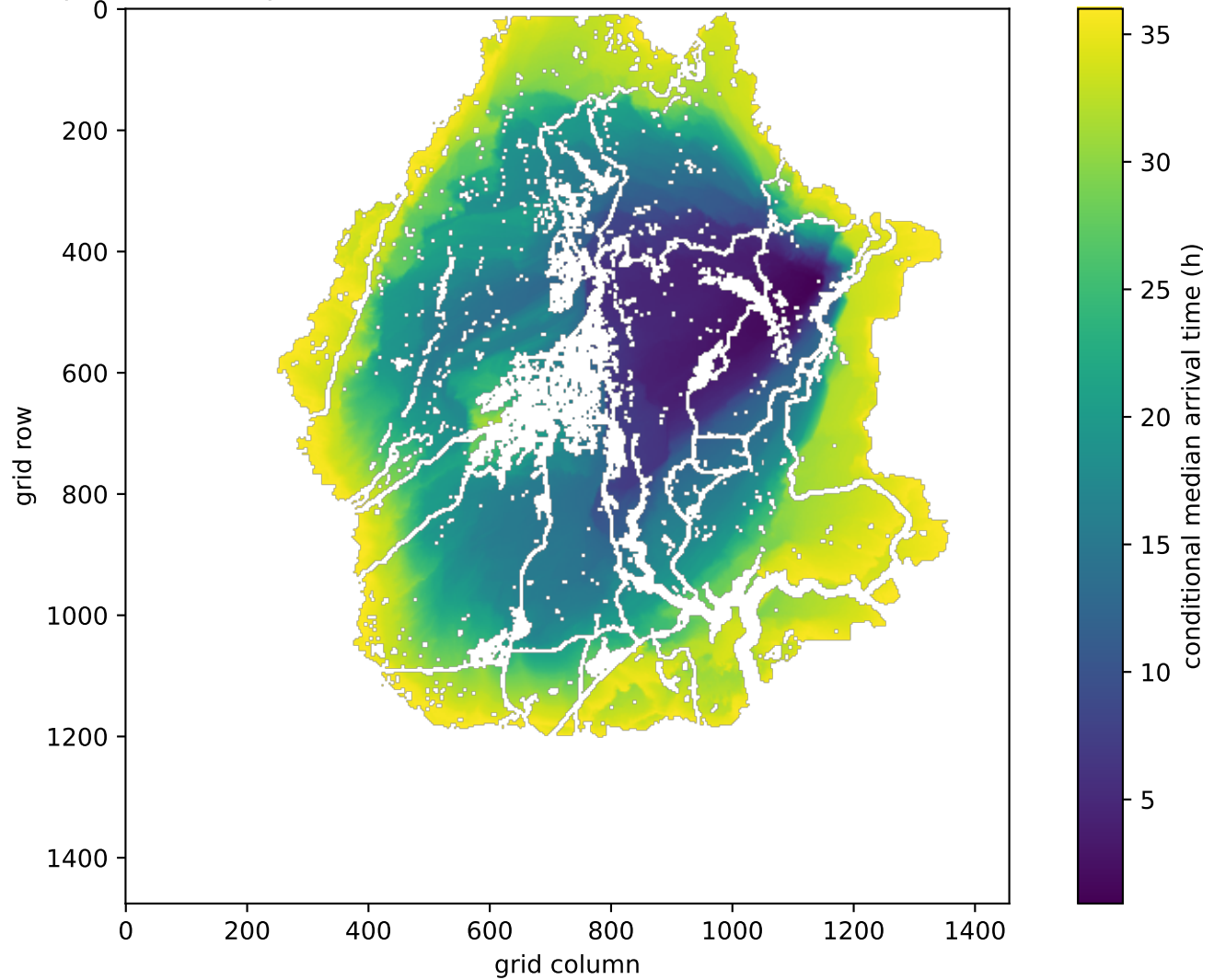
2018 Camp Fire landscape reconstruction: arrival time where at least one member burns
