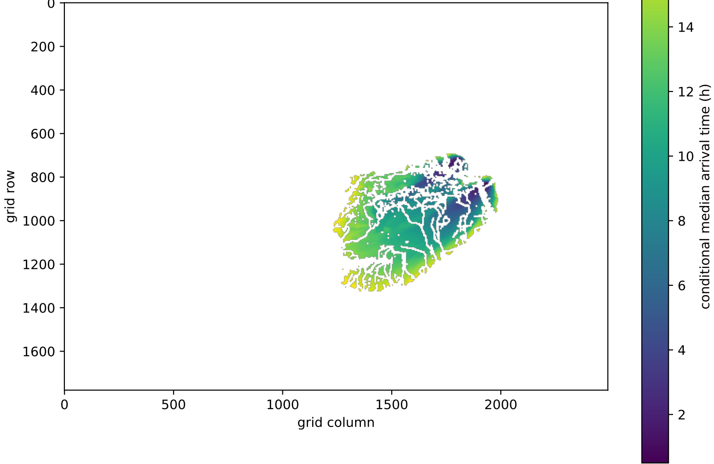
2017 Thomas Fire landscape reconstruction: arrival time where at least one member turns
