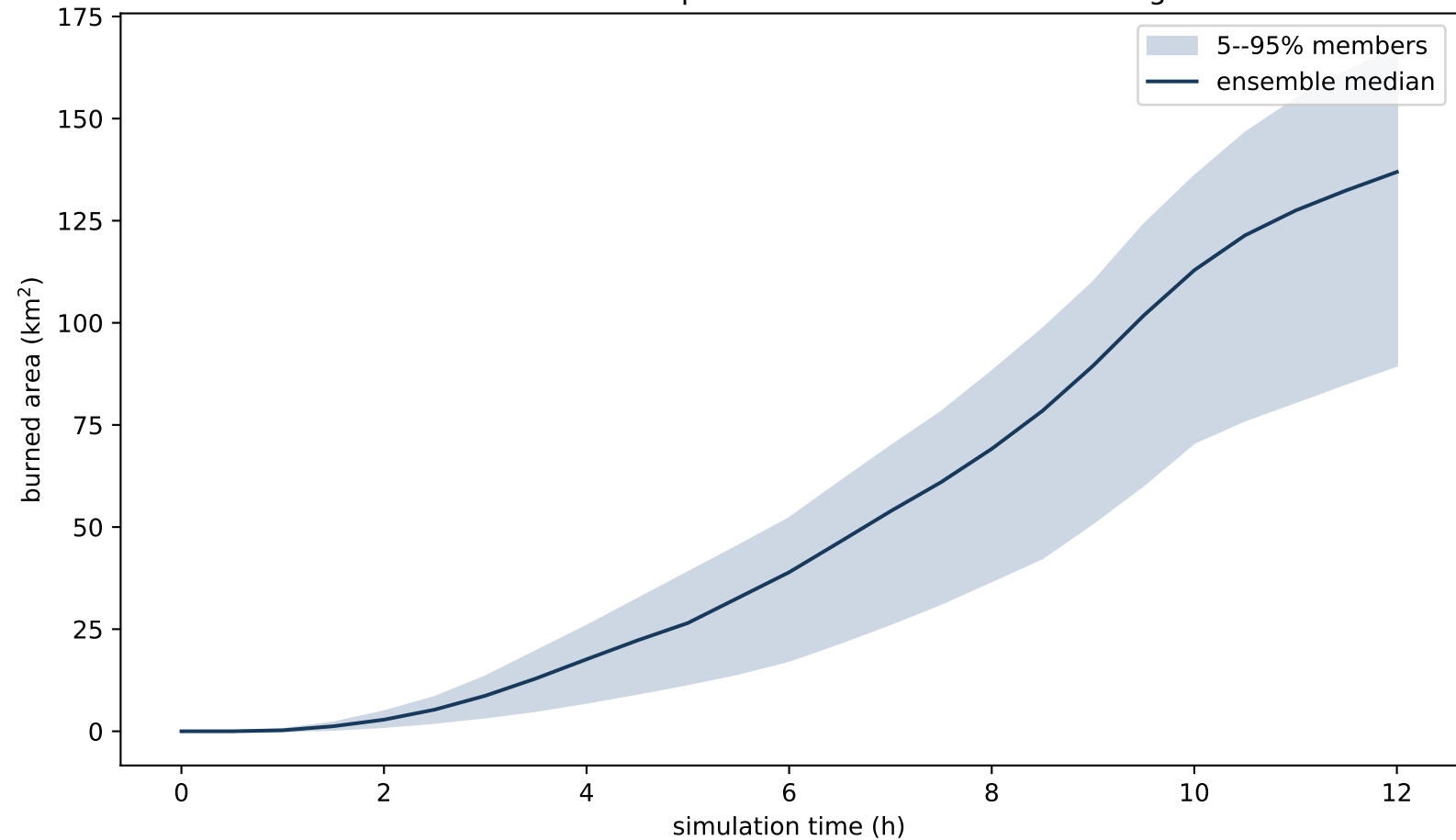
2017 Tubbs Fire landscape reconstruction: burned-area growth
