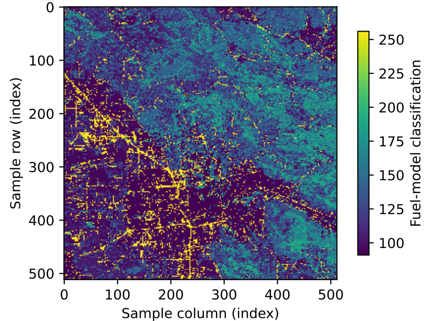
Fuel-model classification
