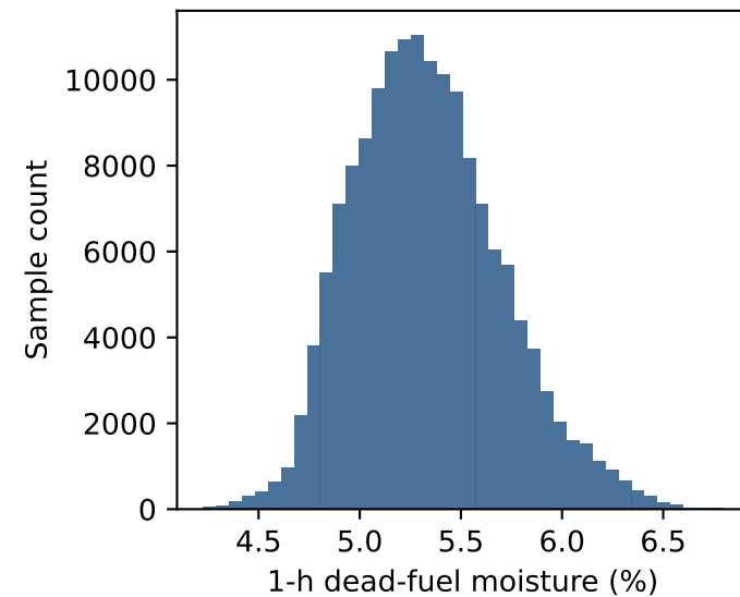
1-h dead-fuel moisture (%)
