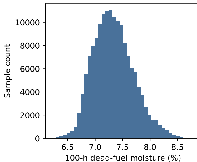
100-h dead-fuel moisture (%)
