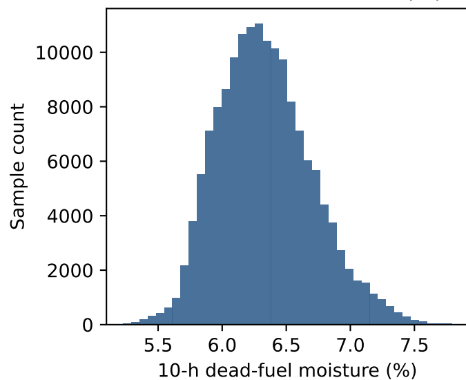
10-h dead-fuel moisture (%)
