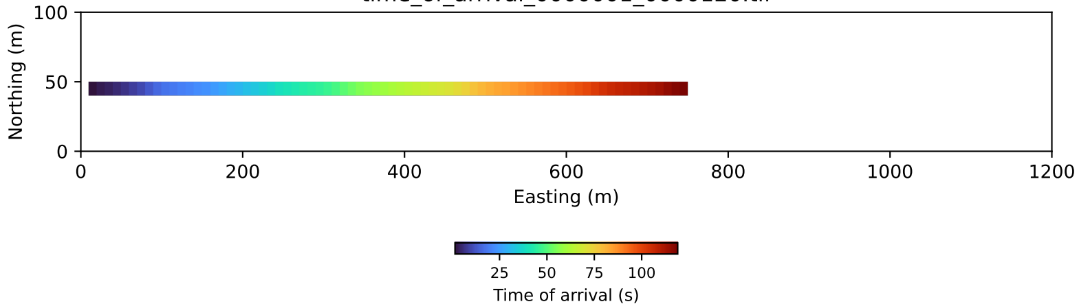
Time-of-arrival field — base case time_of_arrival_0000001_0000120.tif
