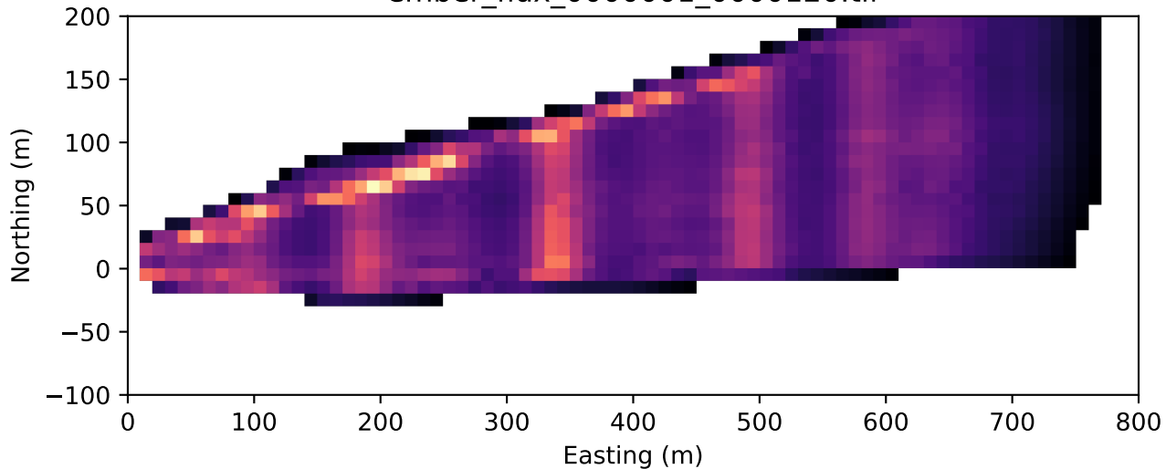
Accumulated firebrand distribution — base case ember_flux_0000001_0000120.tif
