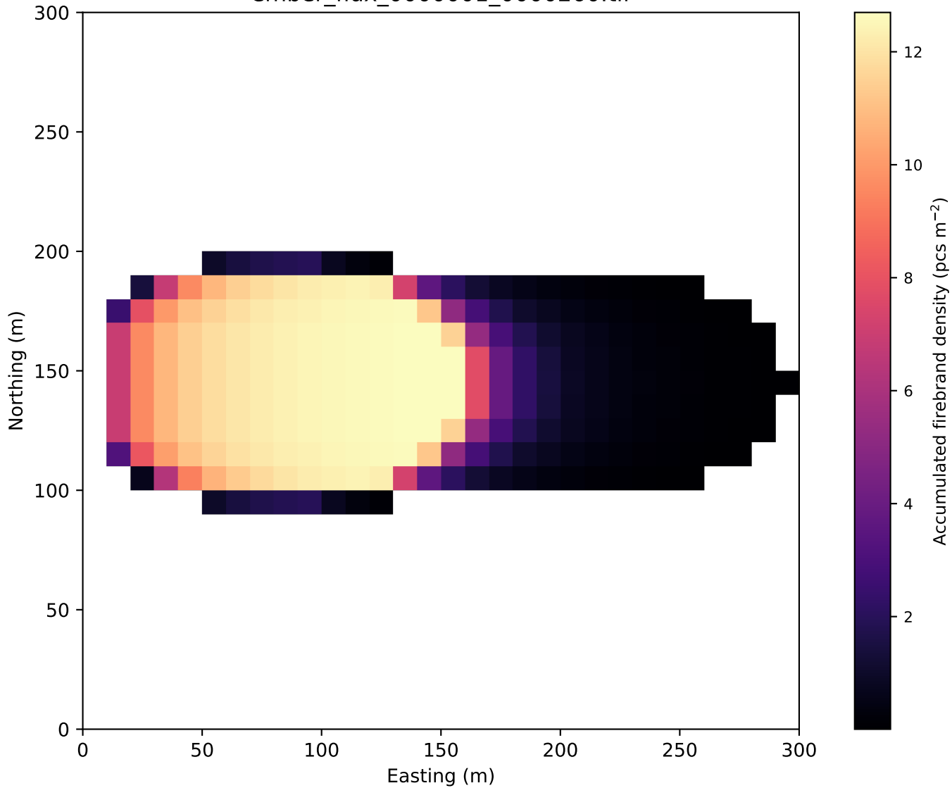
Accumulated firebrand distribution — variants/dx10_consumption_on ember_flux_0000001_0000260.tif
