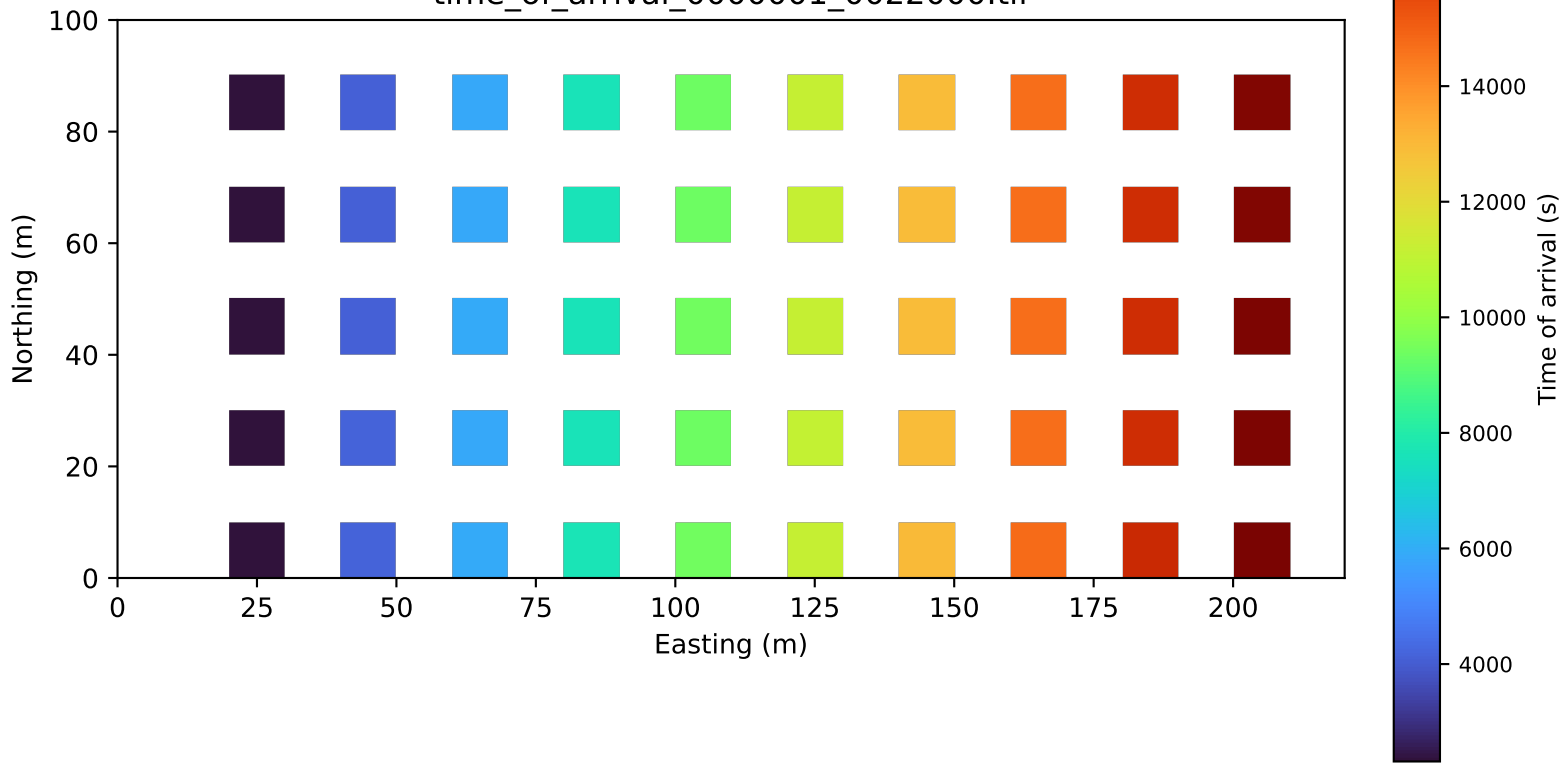
Time-of-arrival field — variants/cfl0p5_dt0p28 time_of_arrival_0000001_0022000.tif
