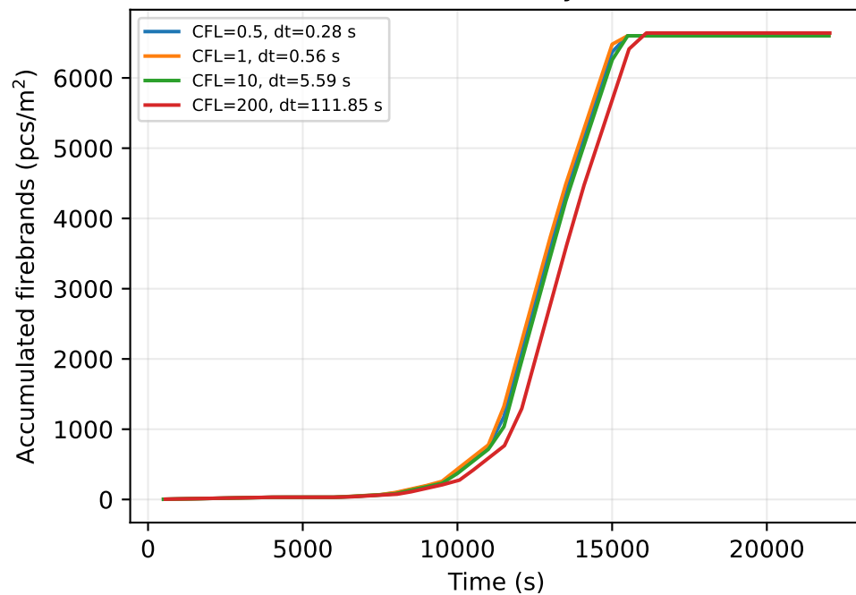
(c) Accumulation history, 140--150 m
