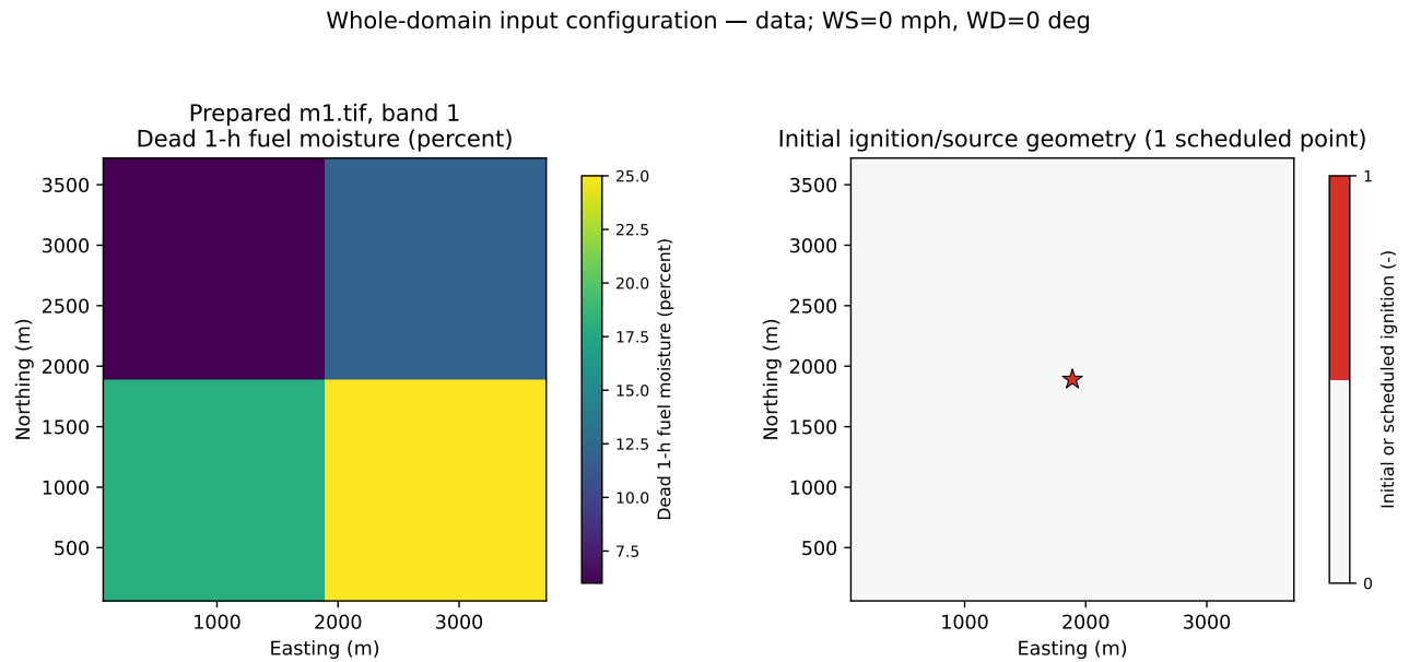
Figure 1: Prepared input conditions from the prescribed spatial fields. Coordinates are in metres; the colorbar identifies the displayed field and its physical units or category. The ignition panel is derived directly from \phi \leq 0 .
