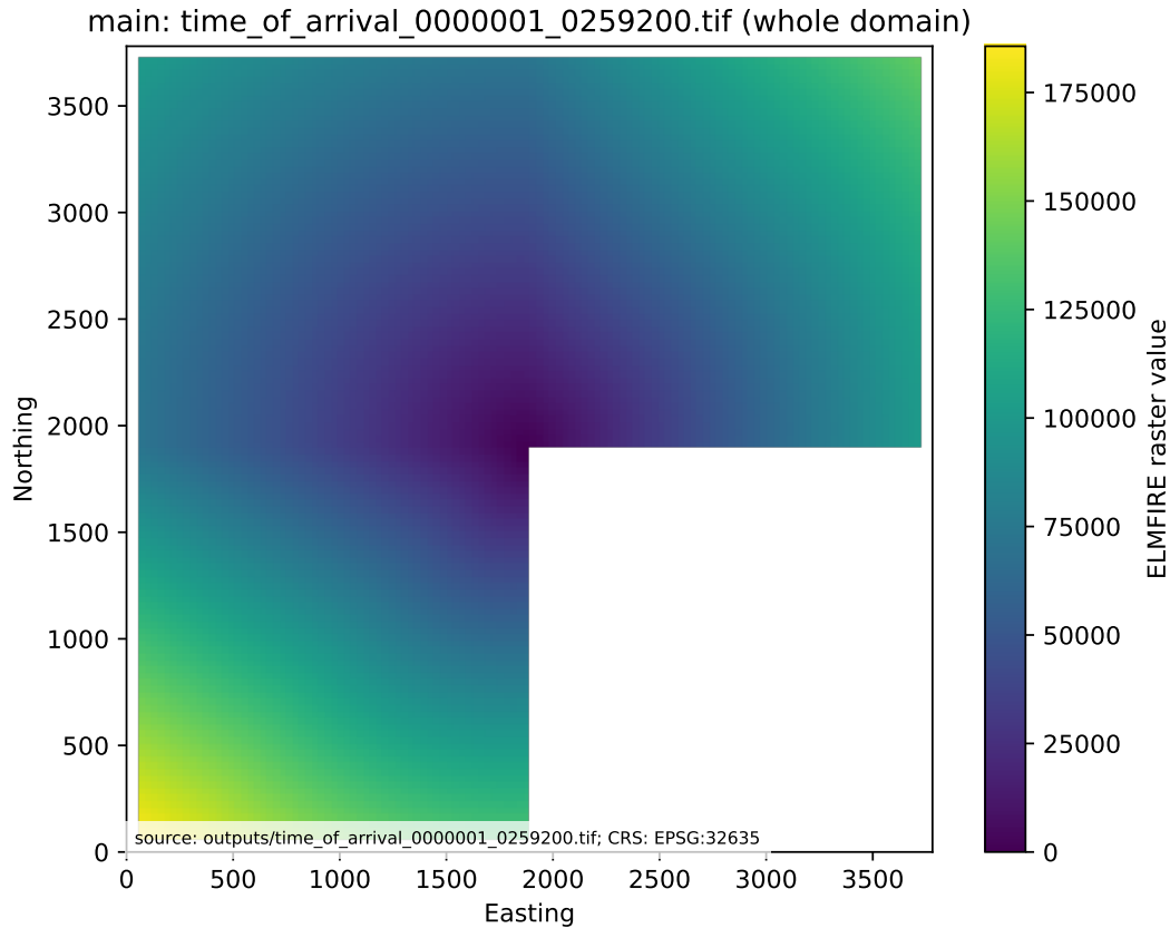
Figure 2: Final whole-domain ELMFIRE time of arrival for the displayed simulation condition, in seconds. The coordinate reference system is stated in the figure. The calculated metrics, not visual appearance, determine acceptance.
