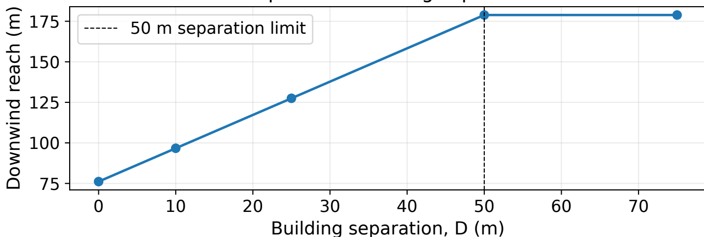
Response to building separation
