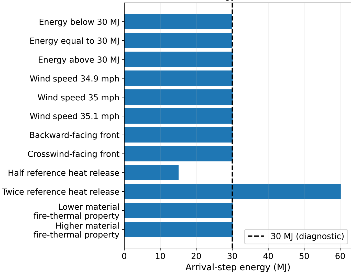
Simulated energy at receiver arrival
