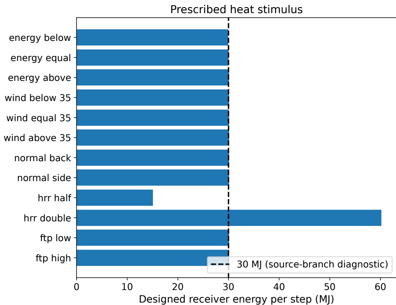
Figure 2: Prescribed receiver energy for all twelve simulation conditions, read from the generated input simulation specification. The dashed line marks the source energy-branch diagnostic, not an acceptance threshold.
