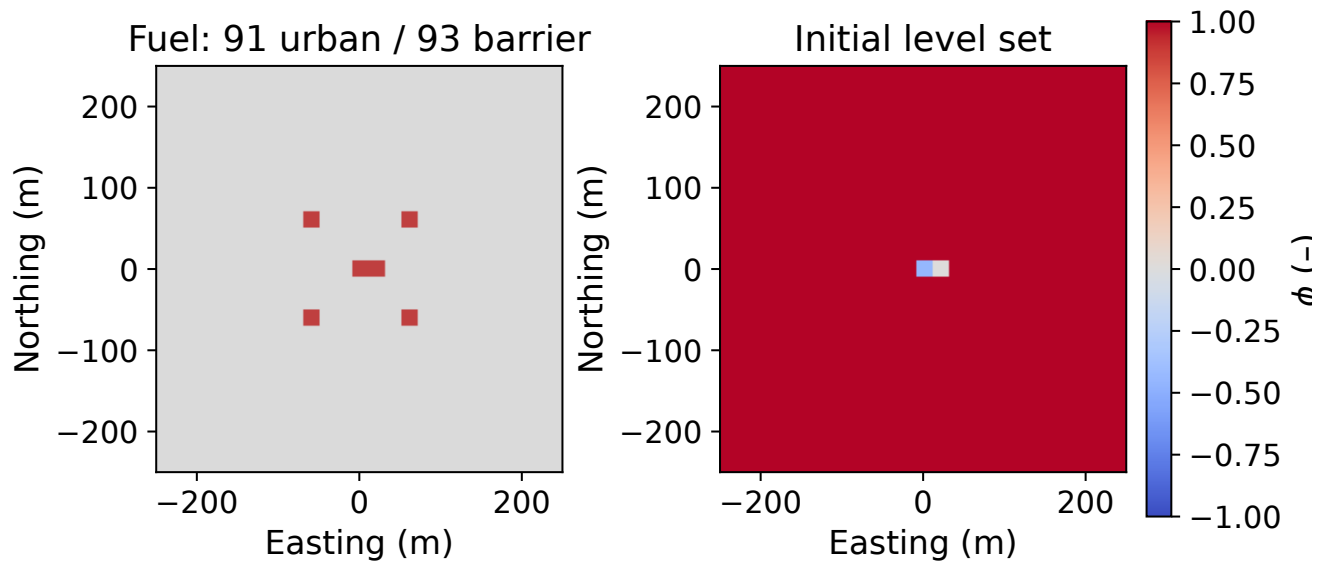
Figure 1: Whole-domain prepared fuel and initial-level-set fields. The separate energy figure shows the designed energy sweep. Coordinates are metres in EPSG:32610; the fields represent the equal-energy condition.
