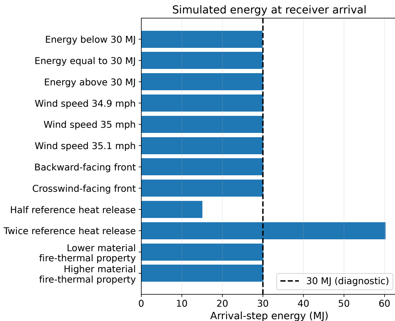
Figure 4: Simulated receiver energy at the selected arrival-step output, calculated from the recorded direct-flame-contact and radiative heat fields. The dashed line identifies the energy-branch transition in the reviewed formulation; it is not an acceptance threshold.
