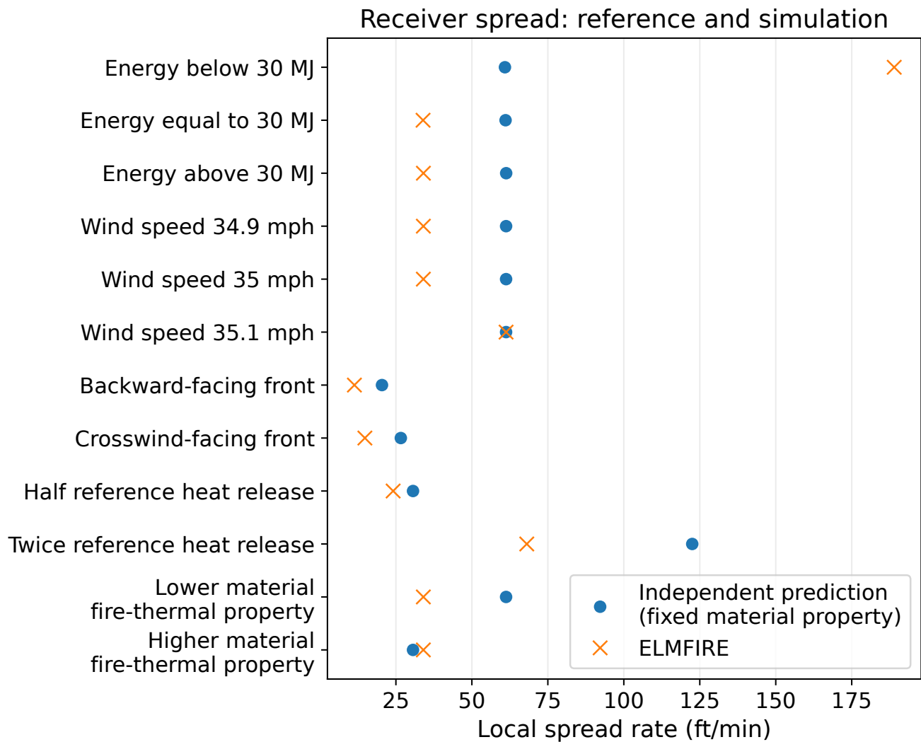
Figure 3: Simulated receiver spread rates and independent predictions for all twelve simulation conditions. The predictions recompute the heat-to-spread relation using the simulated heat stimulus. This comparison isolates the receiver response from differences in the supplied heating; separate figures show the heat stimulus and the spatial result.
