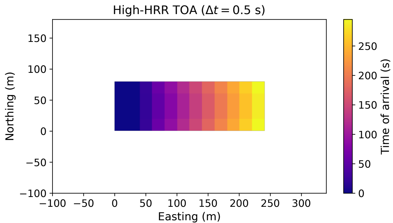
Figure 3: High-HRR exact- t = 300 s TOA for \Delta t = 0.5 s; the exact source raster is recorded in calculated verification and validation metrics.
