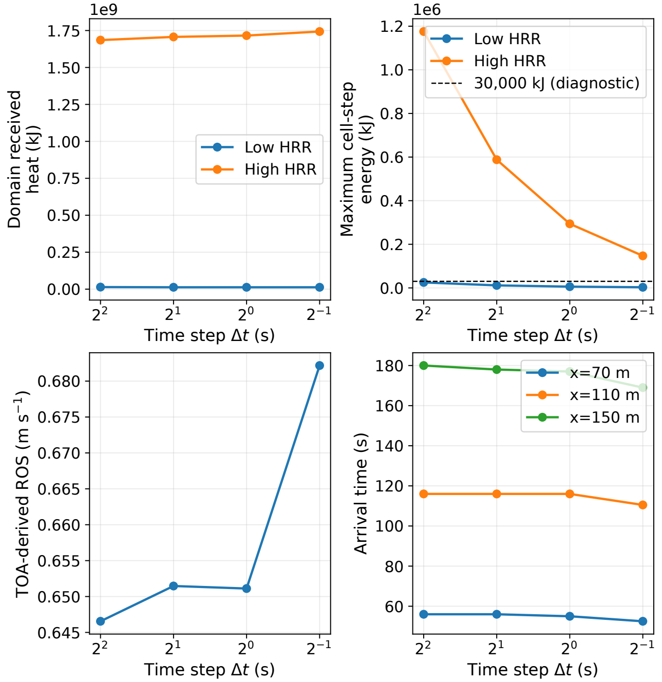
Figure 2: Exact common-time response of heat, sampled FBFM91 energy, ROS, and TOA from completed, input-matched simulations; convergence limits are 5%.
