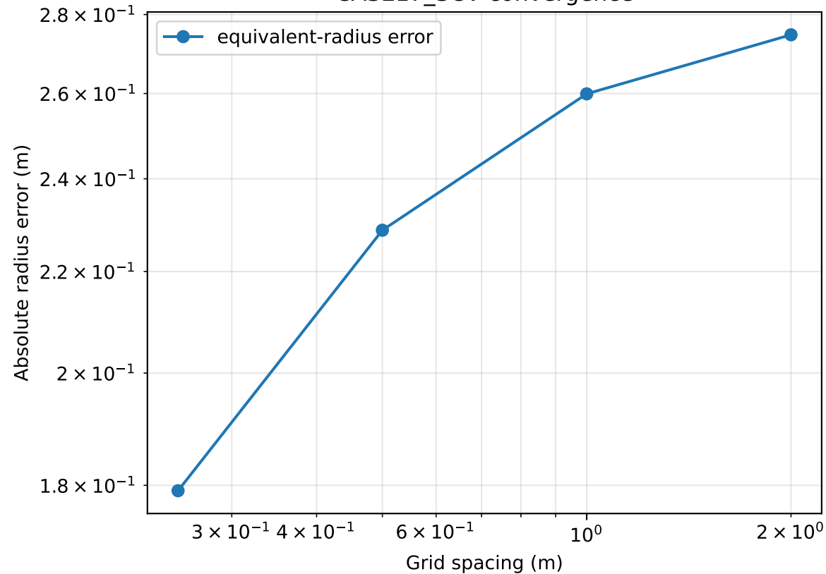
CASE17_SCV convergence
