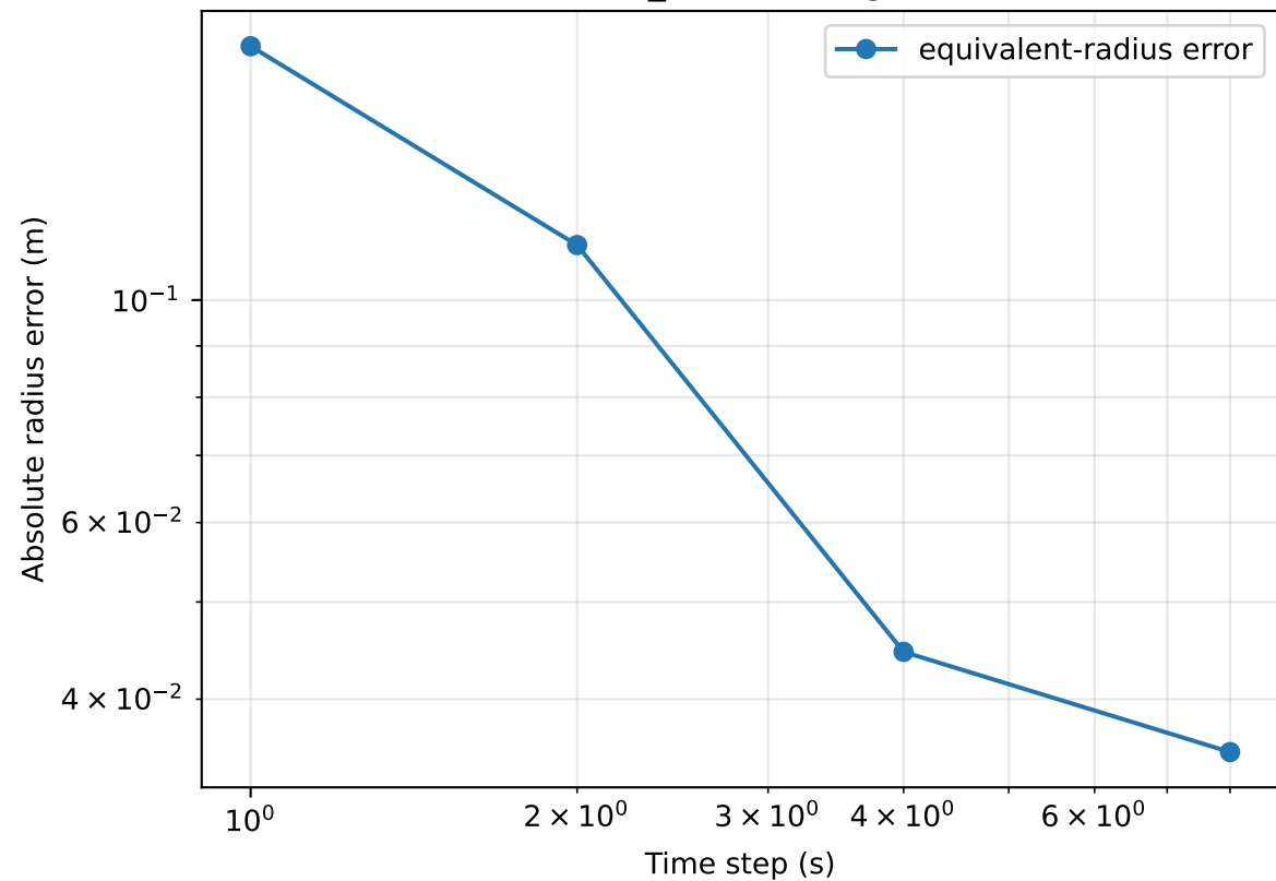
CASE18_TCV convergence
