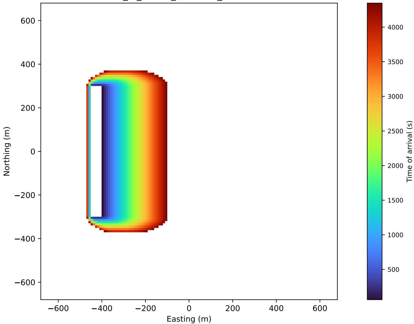
Time-of-arrival field — variants/fuel_188_u_8p0 time_of_arrival_0000001_0004375.tif
