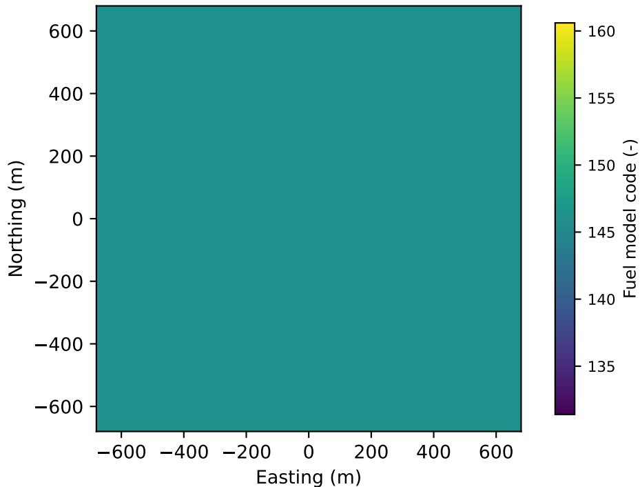
Prepared fbfm40.tif, band 1 Fuel model code (-)
