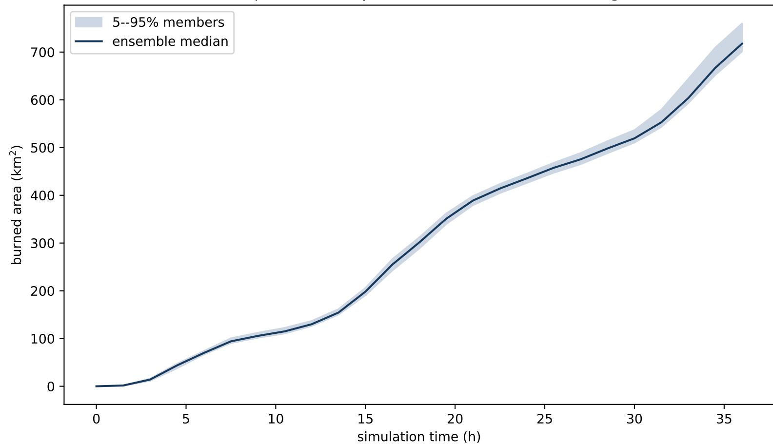
2018 Camp Fire landscape reconstruction: burned-area growth
