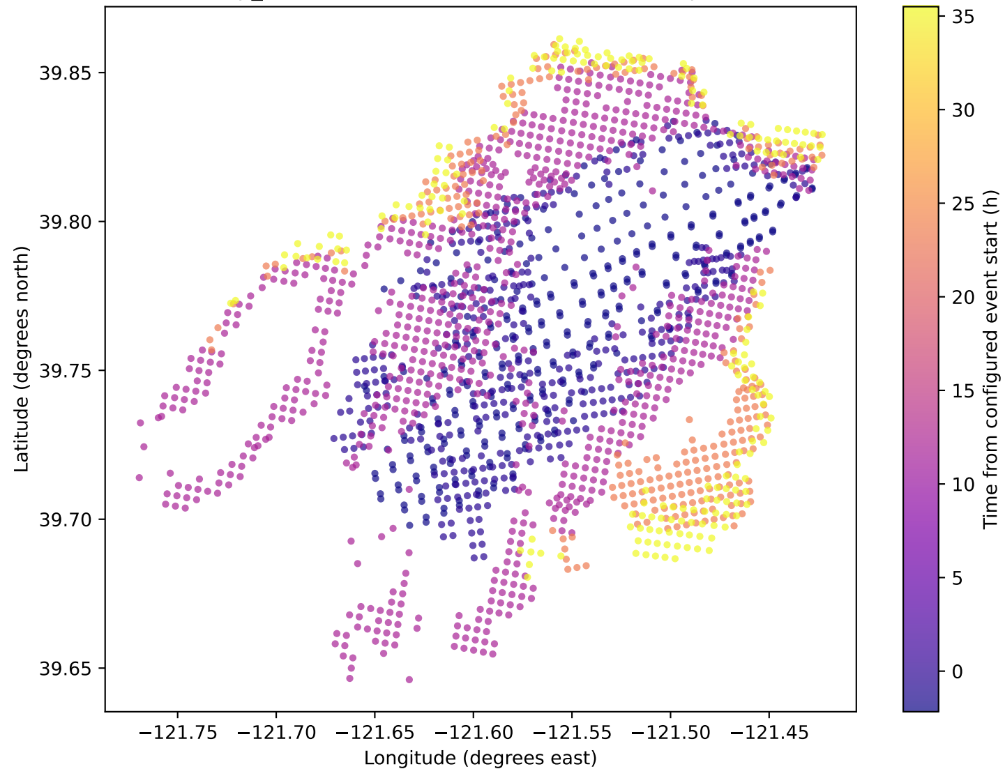
camp_fire: VIIRS detections retained for comparison
