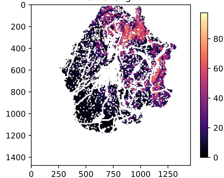
flame length
