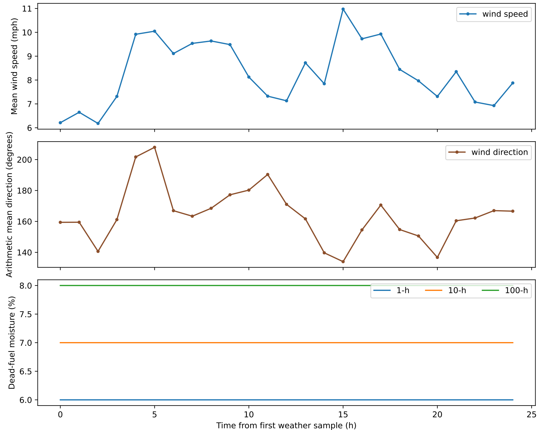
camp_fire: domain-mean weather evolution
