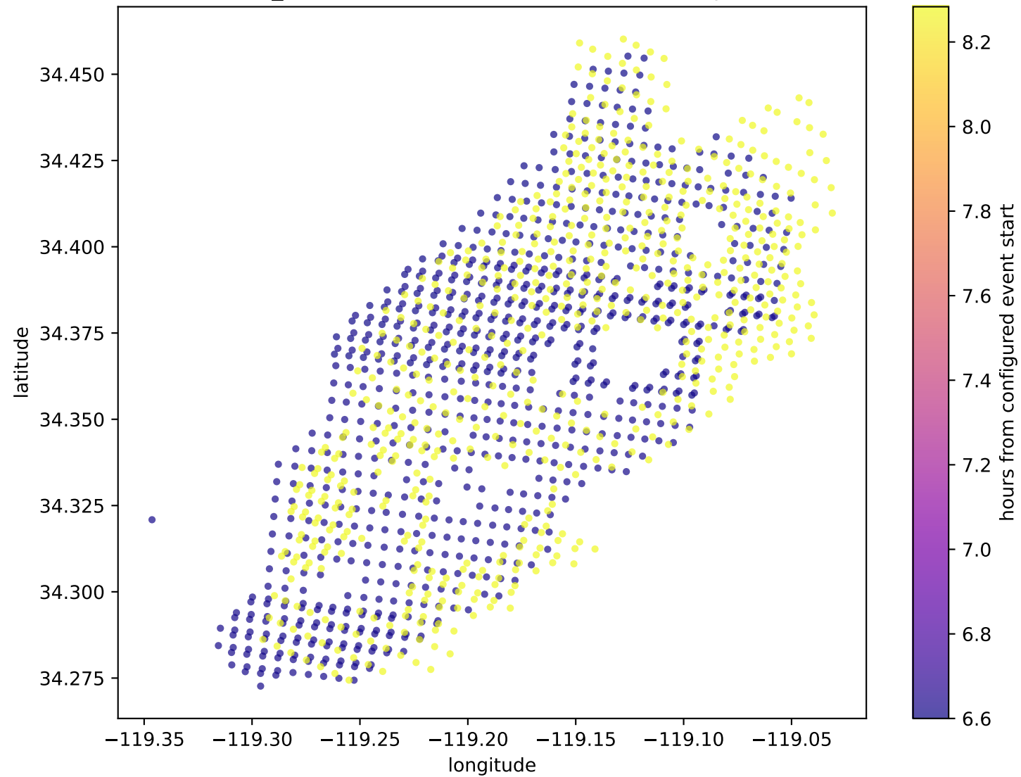
thomas_fire: VIIRS detections retained for comparison
