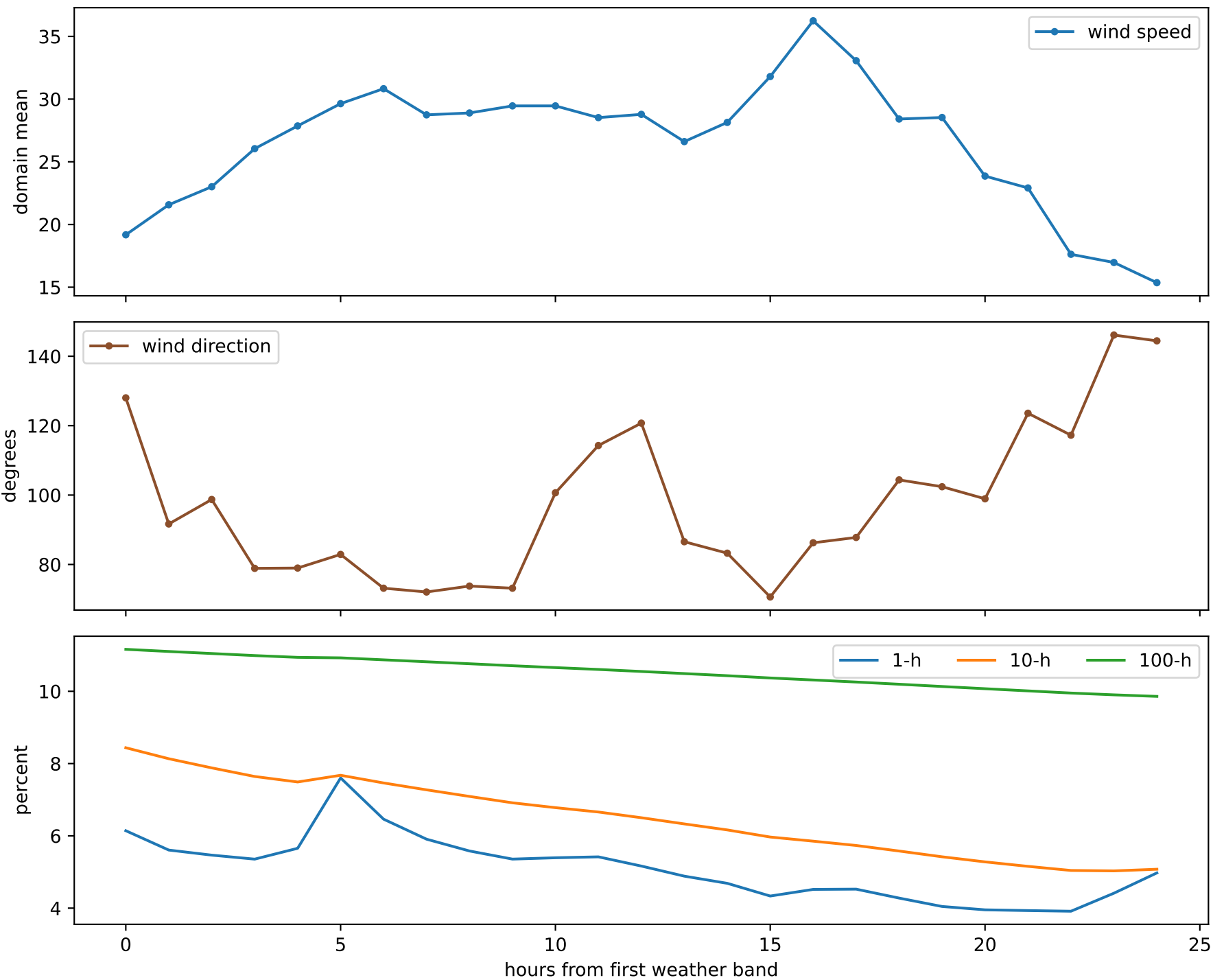
thomas_fire: domain-mean weather evolution
