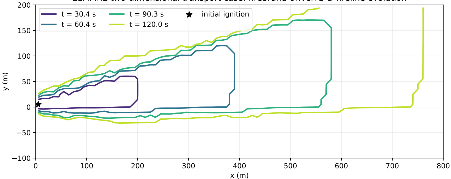
ELMFIRE two-dimensional transport case: firebrand-driven 2-D fireline evolution
