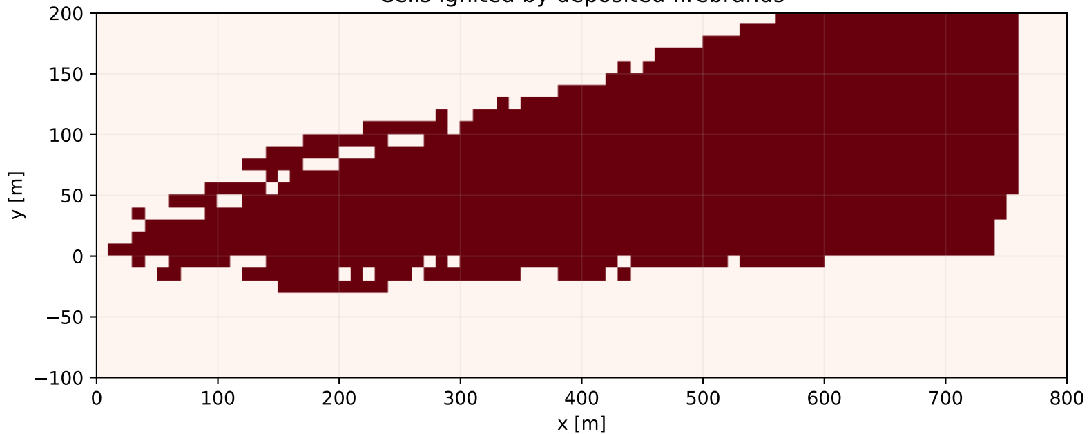
Cells ignited by deposited firebrands
