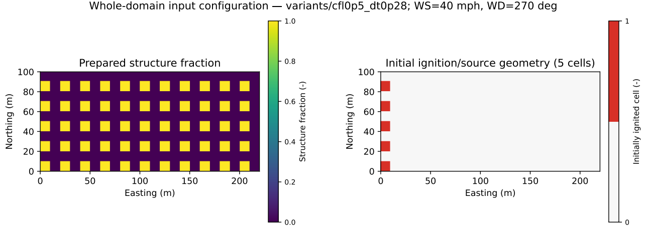
Figure 1: Whole-domain prepared input configuration for the representative simulation condition. The physical domain is shown without the numerical halo; coordinates, configured wind values, fuel or structure layout, and initial ignition/source geometry are identified in the panels.
