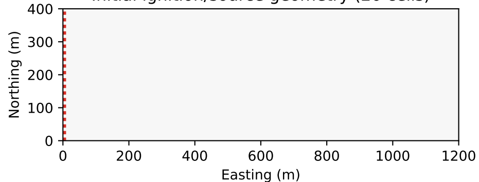
Whole-domain input configuration — variants/dx10; WS=40 mph, WD=270 deg Prepared structure fraction Initial ignition/source geometry (20 cells)
