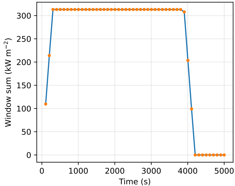
Direct flame contact
