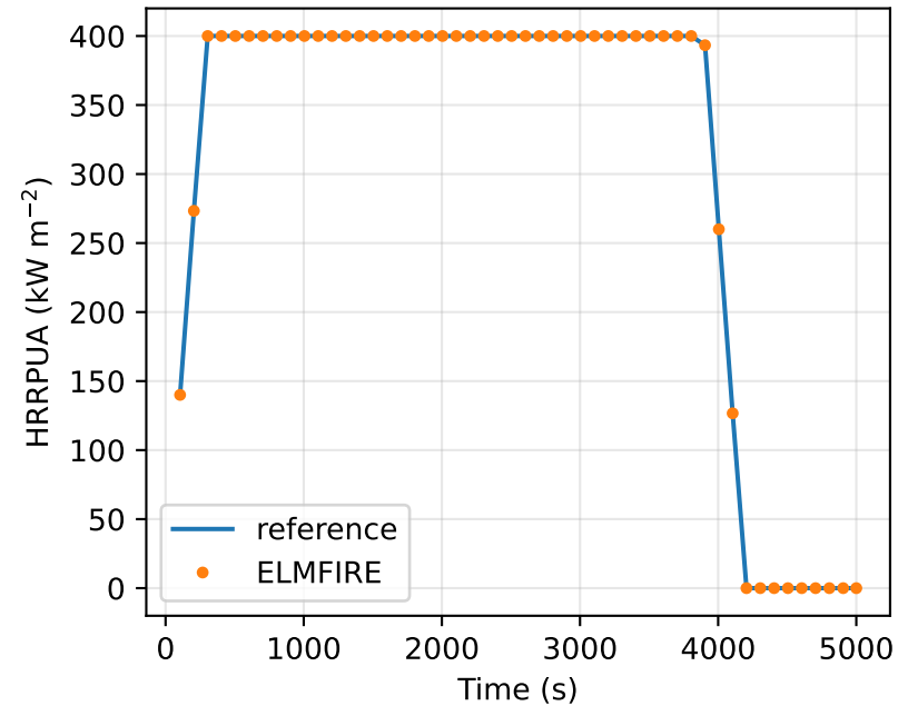
Center-cell HRRPUA
