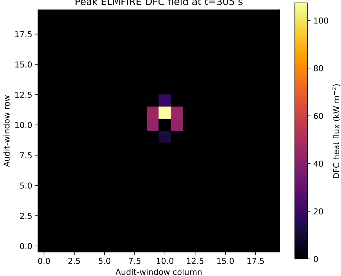
Peak ELMFIRE DFC field at t=305 s
