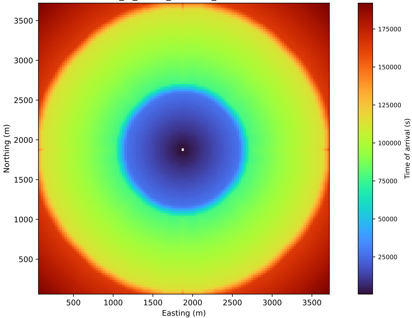
Time-of-arrival field — base case time_of_arrival_0000001_0259200.tif
