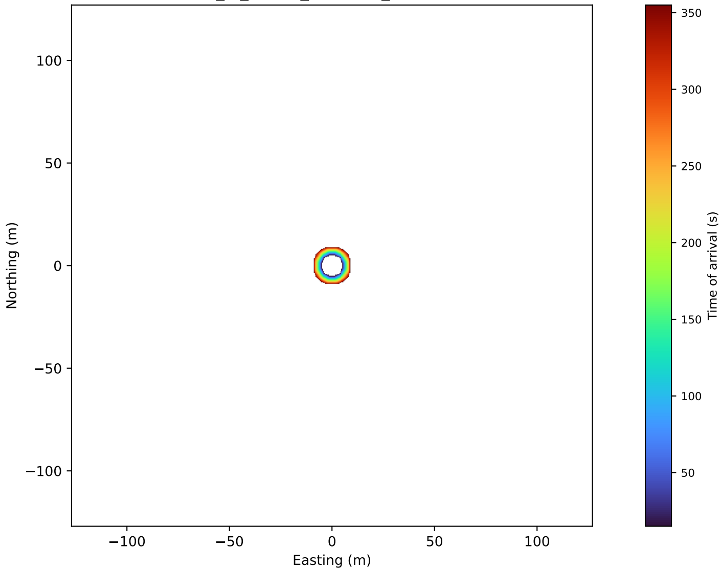
Time-of-arrival field — data/512 time_of_arrival_0000001_0000360.tif
