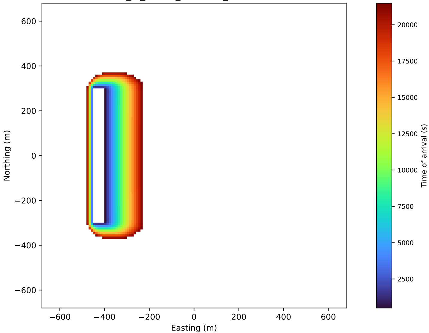
Time-of-arrival field — variants/fuel_123_lh_200 time_of_arrival_0000001_0021609.tif
