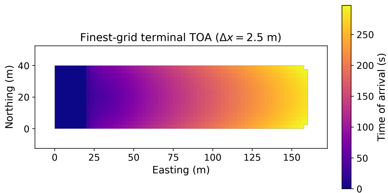
Figure 3: Finest-grid ( \Delta x = 2.5 m) exact- t = 300 s TOA from the unique terminal field for this simulation condition.
