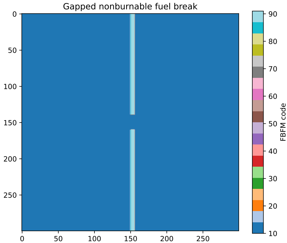
Figure 1: Prescribed fuel-model classification with an opening in the nonburnable strip. Coordinates are grid-cell indices on the 5 m grid, and the color scale identifies the fuel-model codes.
