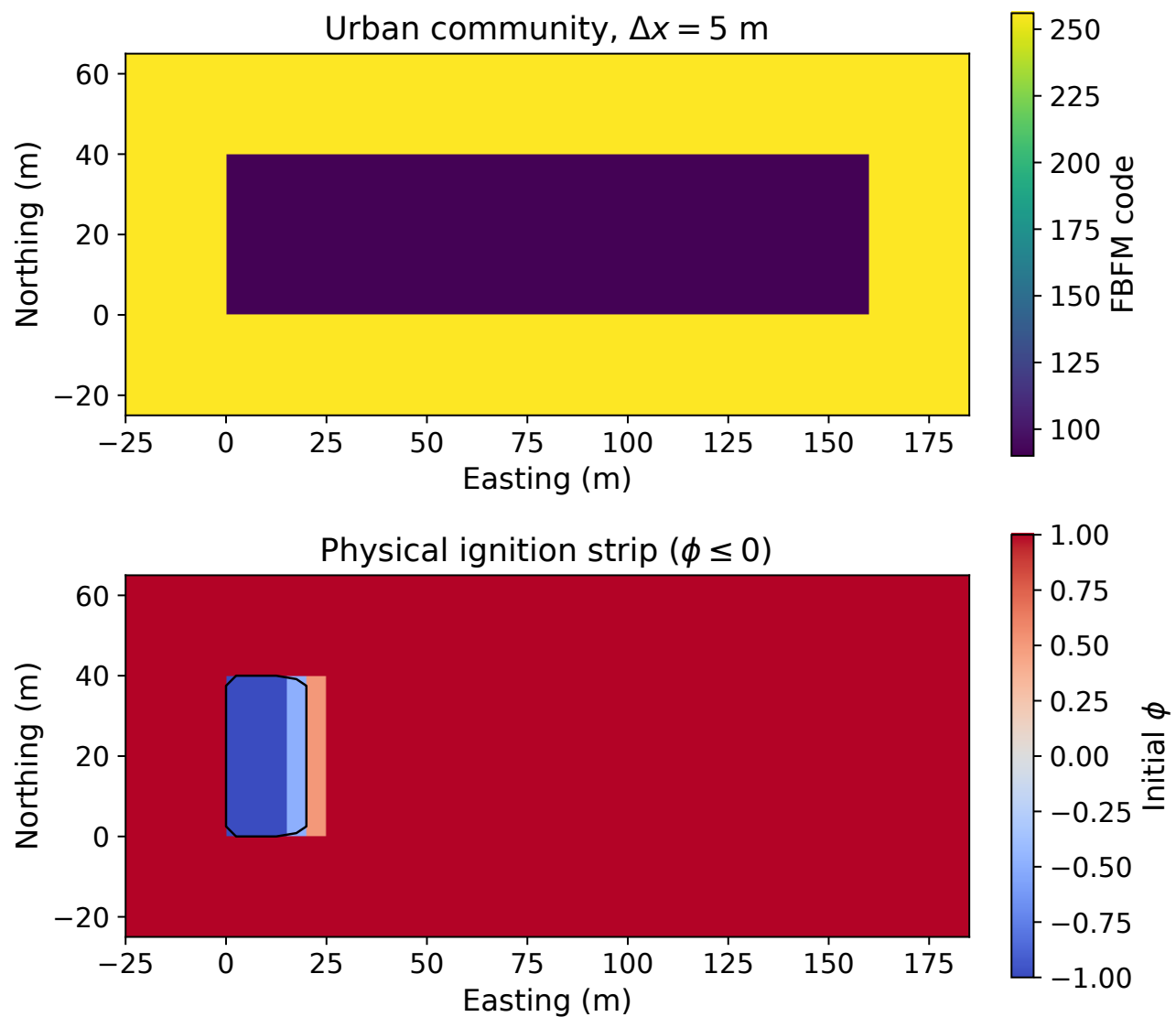
Figure 1: Mechanically rendered fuel-model classification and level-set field; this is the representative 5-m prepared grid, not a simulation result.
