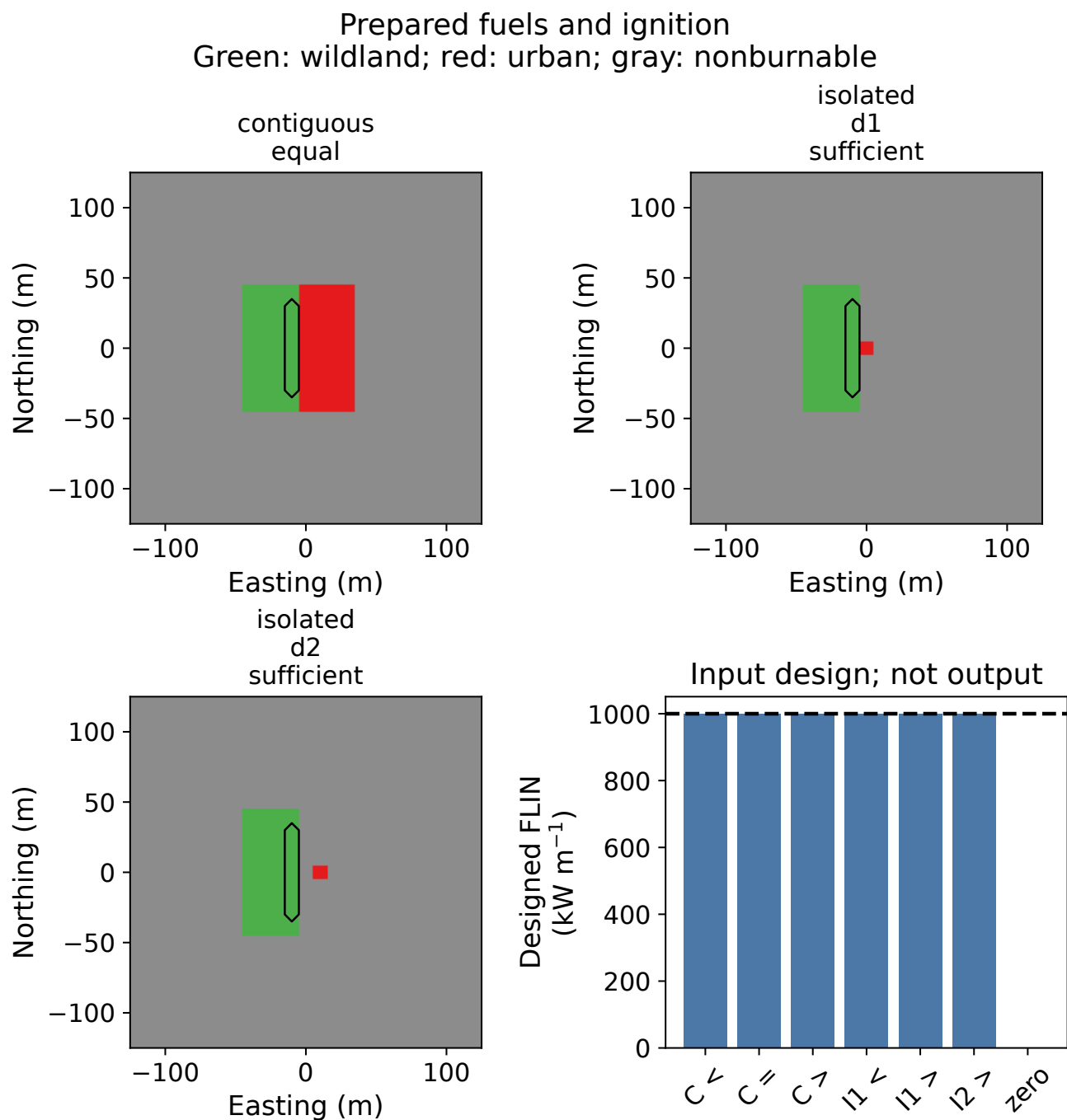
Figure 1: Prepared contiguous and isolated fuel topologies and binary32 source-FLIN design. Green is FBFM01, red is FBFM91, gray is FBFM93, and the black contour marks the seven-cell initial source.
