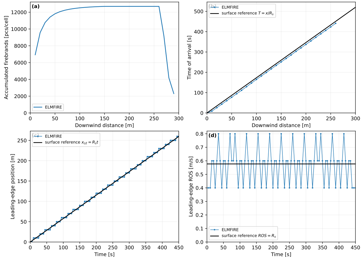
Figure 3: Long-delay surface-dominated simulation condition. The leading edge remains close to the surface-spread characteristic despite continued firebrand deposition.
