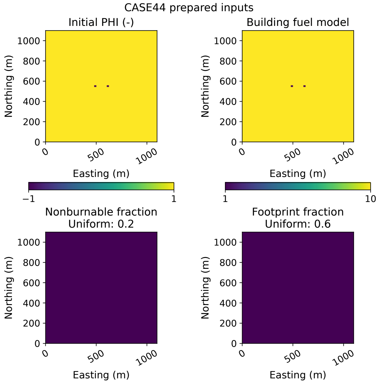
Figure 2: Prepared two-source configuration read back from generated GeoTIFFs. Source model IDs override the uniform target-table ID only at the two initially burning cells.
