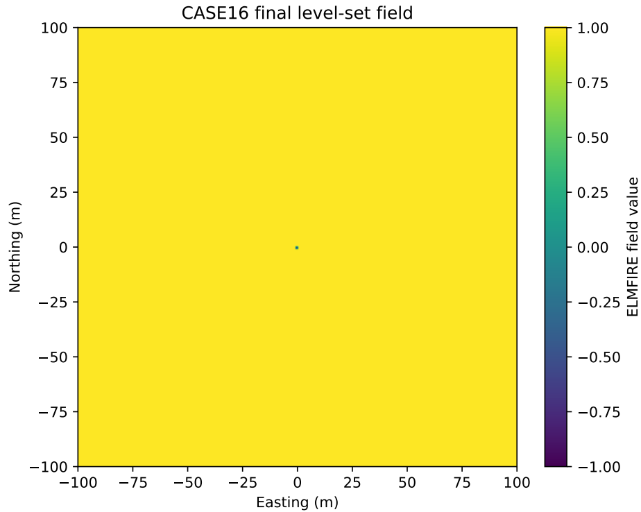
Figure 2: Final whole-domain signed level-set field for the completed zero-spread simulation condition at the final output time. Values are dimensionless; the generated table supplies the rate and confinement limits.
