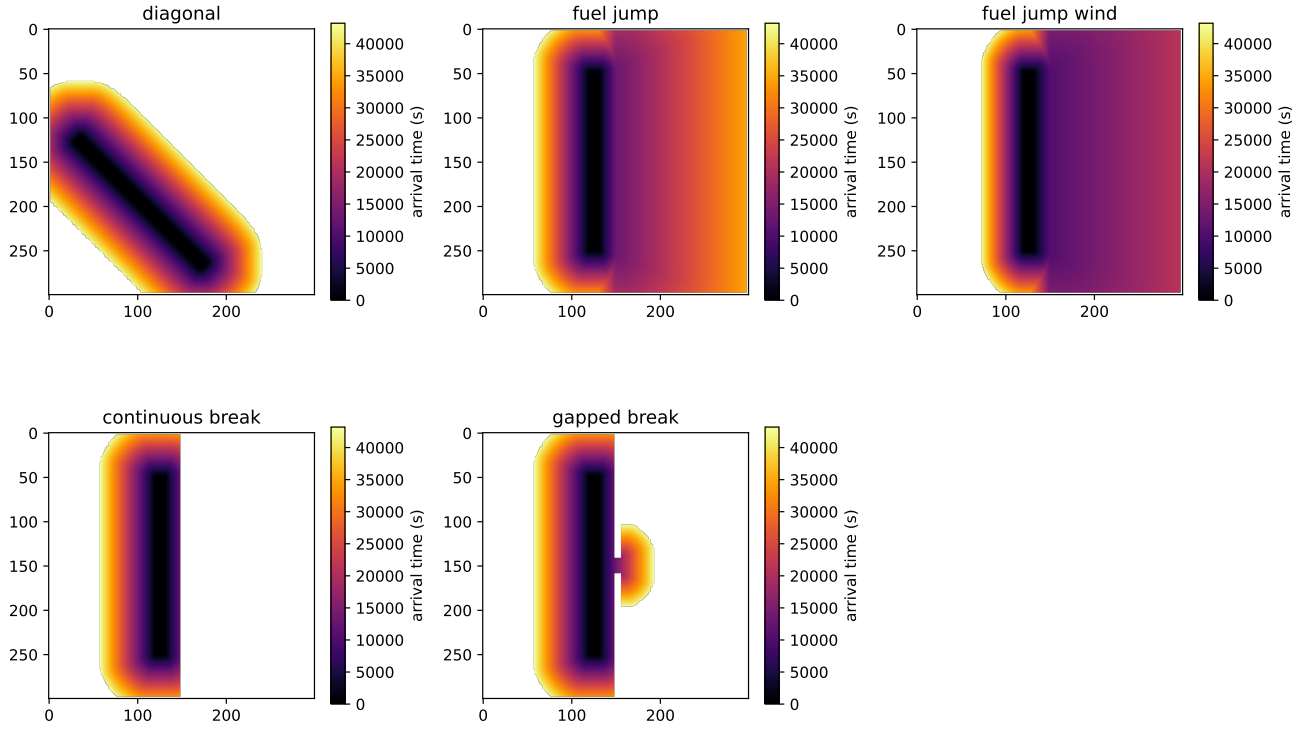
Figure 2: Time-of-arrival fields for all planar-front simulation conditions.
