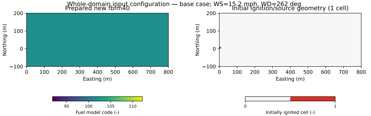
Figure 1: Whole-domain prepared input configuration for the representative simulation condition. The physical domain is shown without the numerical halo; coordinates, configured wind values, fuel or structure layout, and initial ignition/source geometry are identified in the panels.
