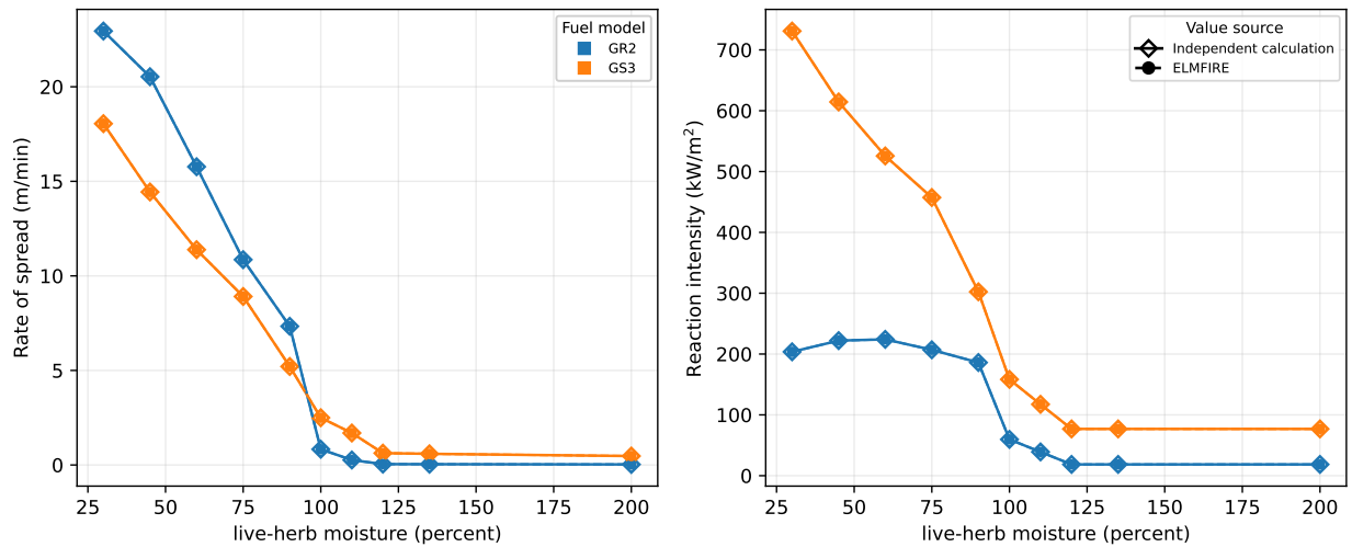
Figure 2: Independent calculations (open diamonds, solid lines) and ELMFIRE predictions (filled circles, dashed lines) for the dynamic-curing response. Each fuel-model pair uses the same color.
