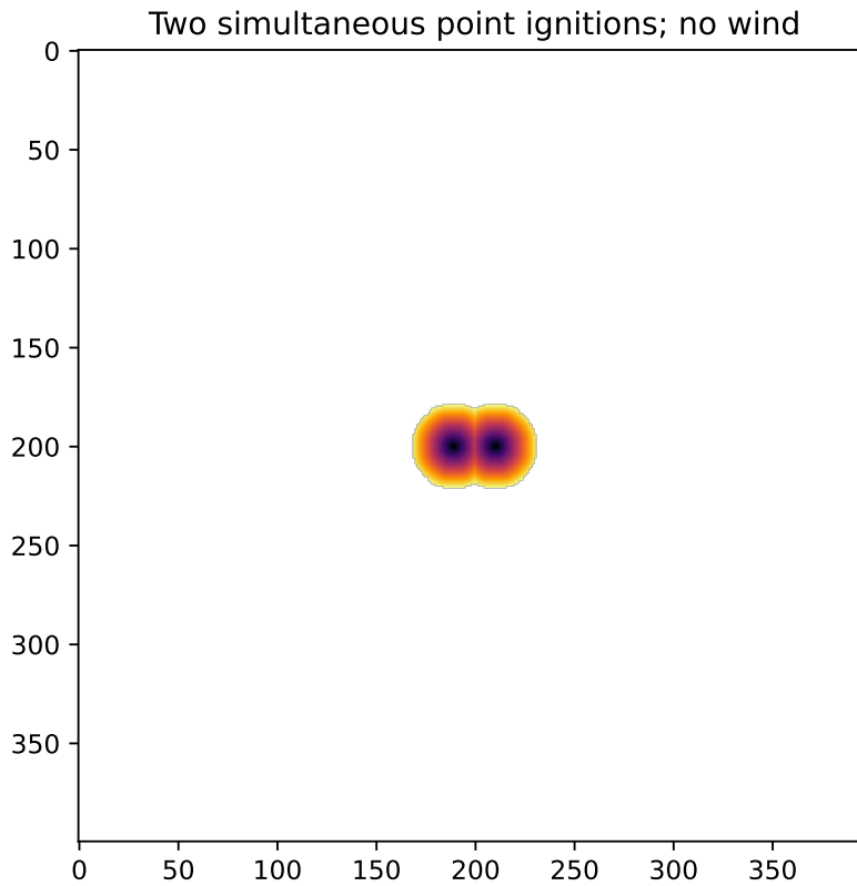
Figure 1: Prescribed initial level-set geometry for two simultaneous ignitions without wind. Coordinates are grid-cell indices on the 5 m grid; the field is dimensionless.
