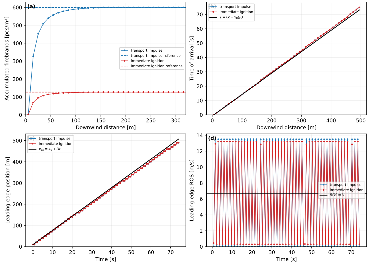
Figure 3: Steady-transport and immediate-ignition observables from actual ELMFIRE outputs. Solid colored curves identify the two controlled simulation conditions; black or color-matched reference curves show the derived analytical behavior.
