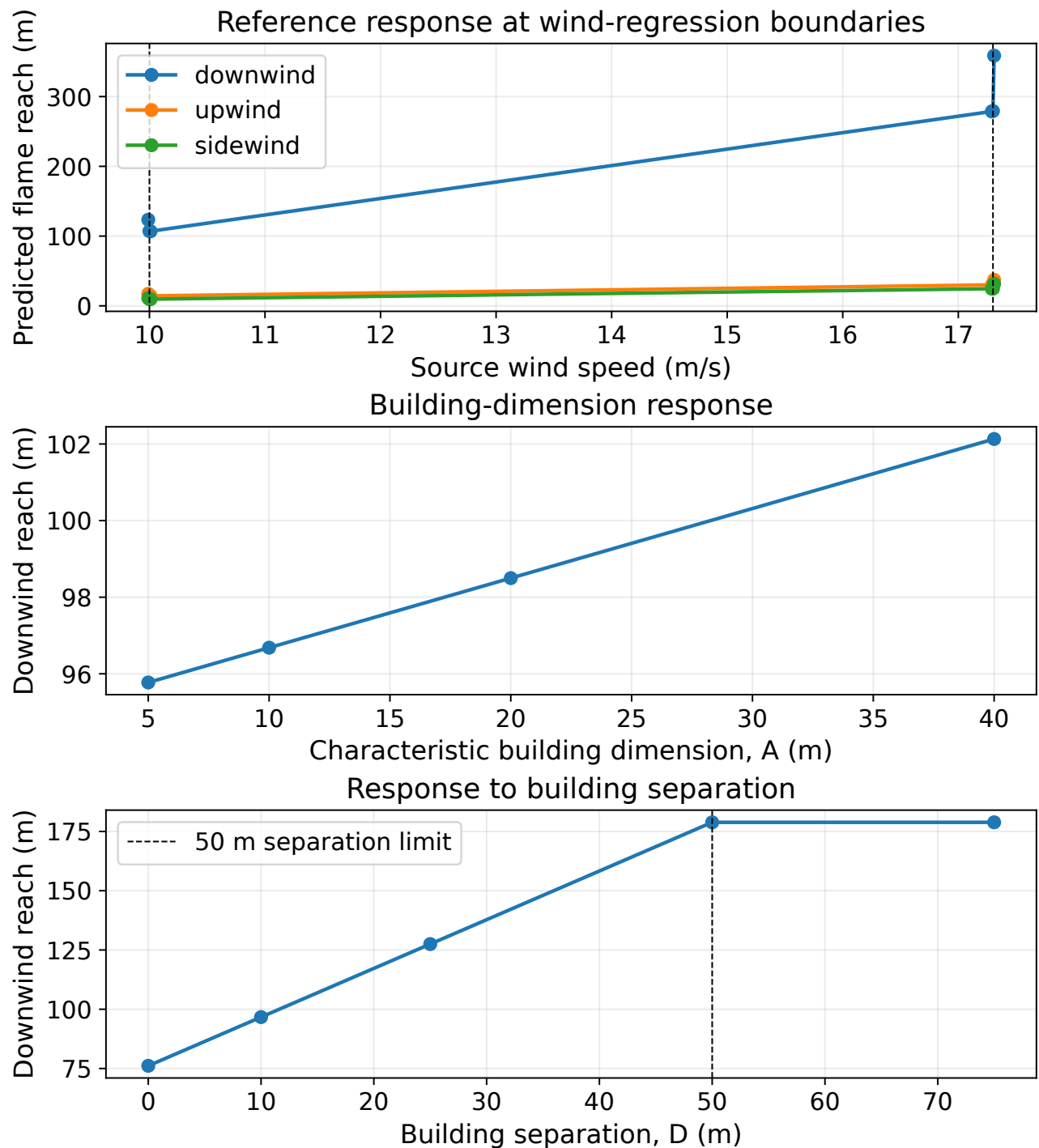
Figure 1: Intended-model reference calculation for the branch, characteristic building dimension, and separation sweeps. These are predicted values, not ELMFIRE output.
