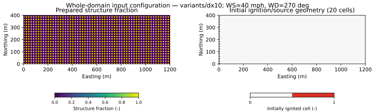
Figure 1: Whole-domain prepared input configuration for the representative simulation condition. The physical domain is shown without the numerical halo; coordinates, configured wind values, fuel or structure layout, and initial ignition/source geometry are identified in the panels.
