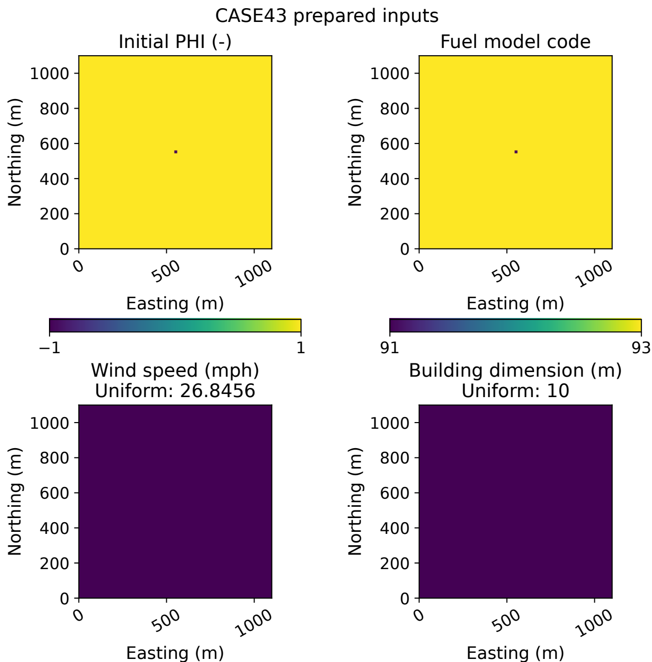
Figure 2: Whole-domain prepared configuration generated from the the 270-degree wind-direction condition GeoTIFF inputs. The single negative PHI cell is the initial WU-E source; FBFM93 and zero adjustment prevent secondary spread.
