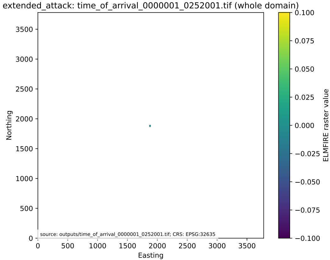
Figure 2: Whole-domain extended-attack time of arrival in seconds when a case-specific output figure exists. It provides spatial context but cannot substitute for the scalar containment and end-time metrics.
