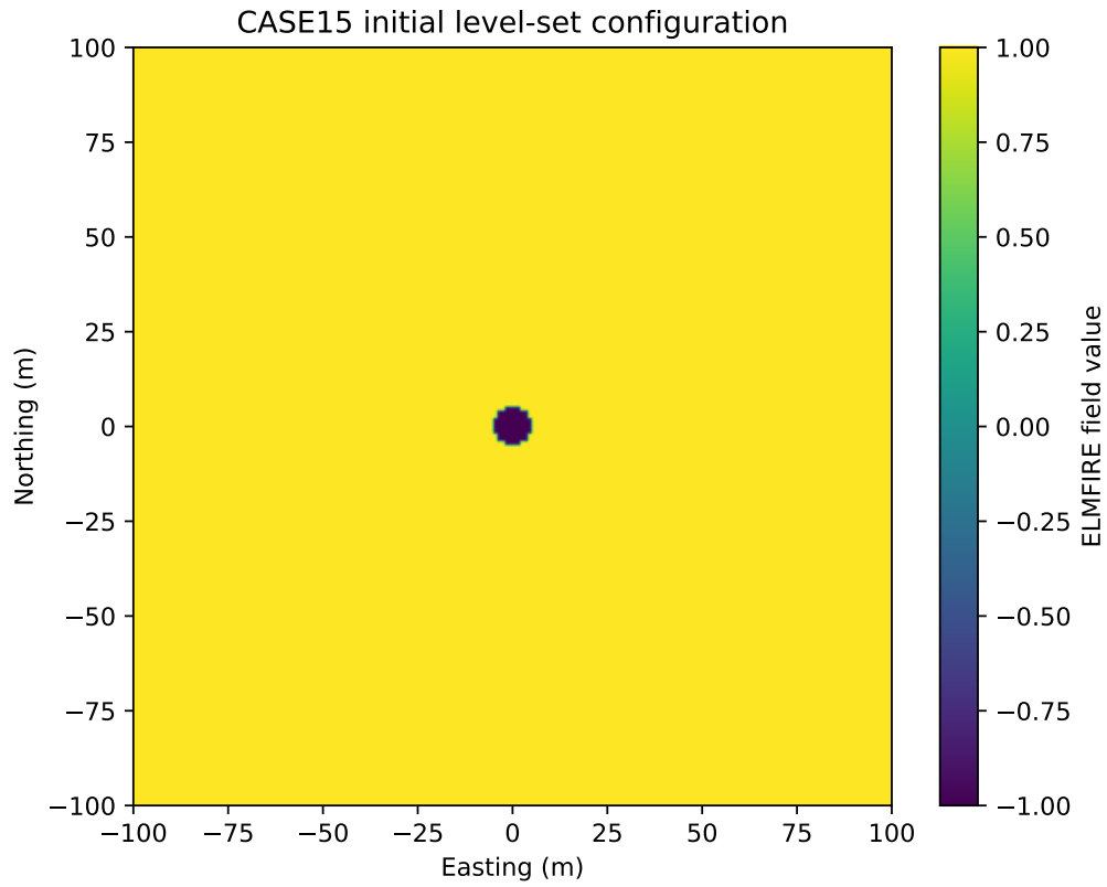
Figure 1: Prepared input conditions from the prescribed spatial fields. Coordinates are in metres; the colorbar identifies the displayed field and its physical units or category. The ignition panel is derived directly from \phi \leq 0 .
