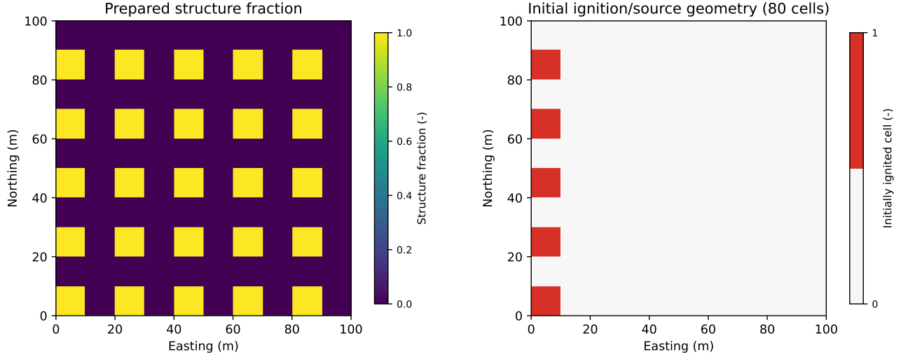
Figure 1: Whole-domain prepared input configuration for the representative simulation condition. The physical domain is shown without the numerical halo; coordinates, configured wind values, fuel or structure layout, and initial ignition/source geometry are identified in the panels.
