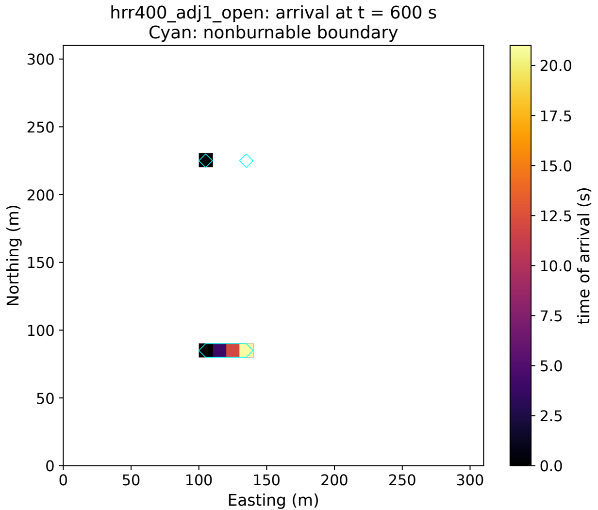
Figure 3: Actual whole-domain time of arrival for the open configuration with heat-release rate per unit area 400 and adjustment factor 1 at 600 s; nodata remains blank and the cyan line marks the FBFM99 boundary. The selected field is the unique terminal arrival-time result for this simulation condition.
