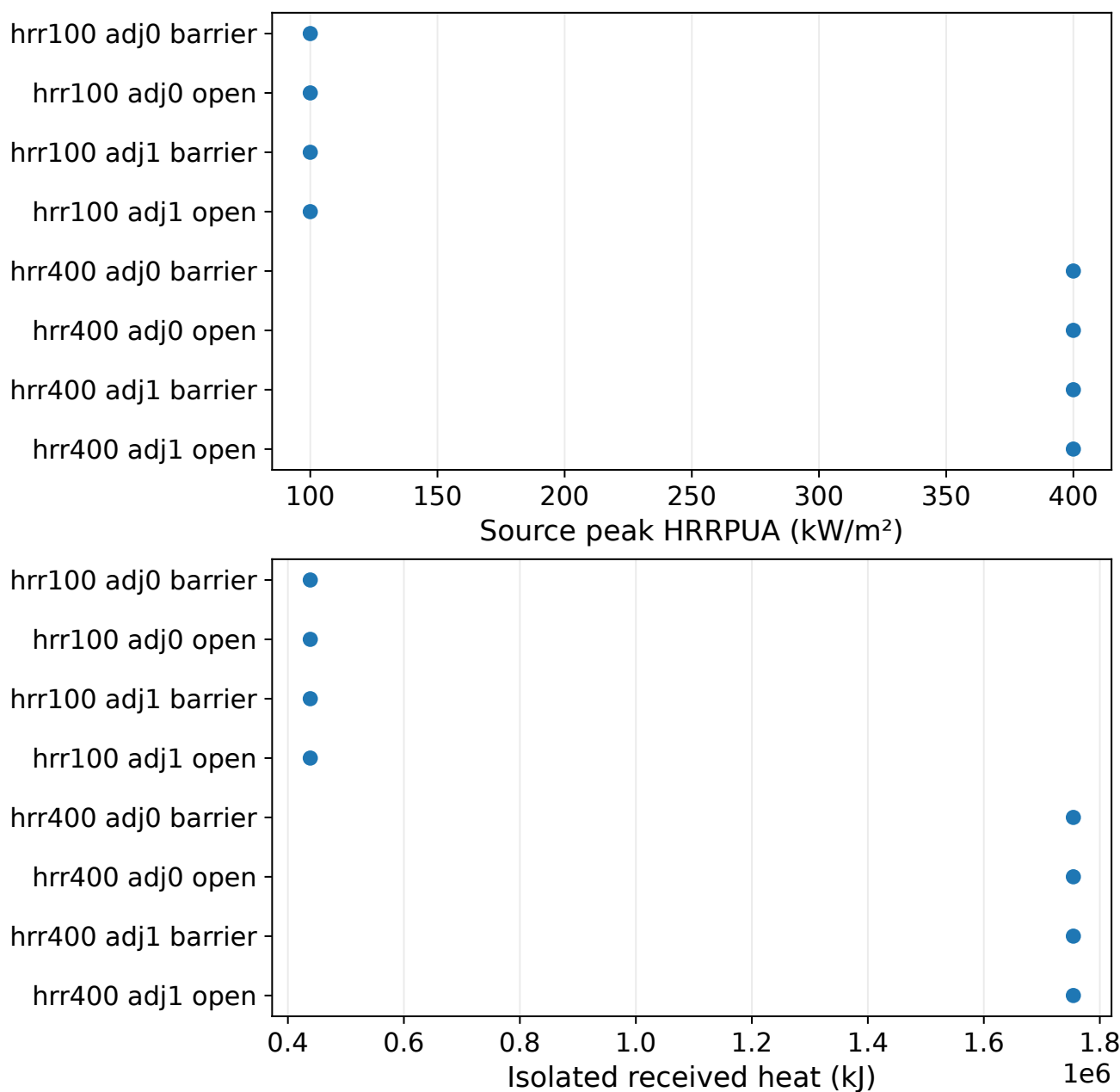
Figure 2: Actual case-specific source HRR and isolated-cell accumulated heat for all eight simulation conditions through 600 s. Values are read from ELMFIRE GeoTIFF outputs; they are not synthetic reference curves. Amplitude-ratio limits are 1% for source HRR and 2% for heat. Arrival times are shown separately.
