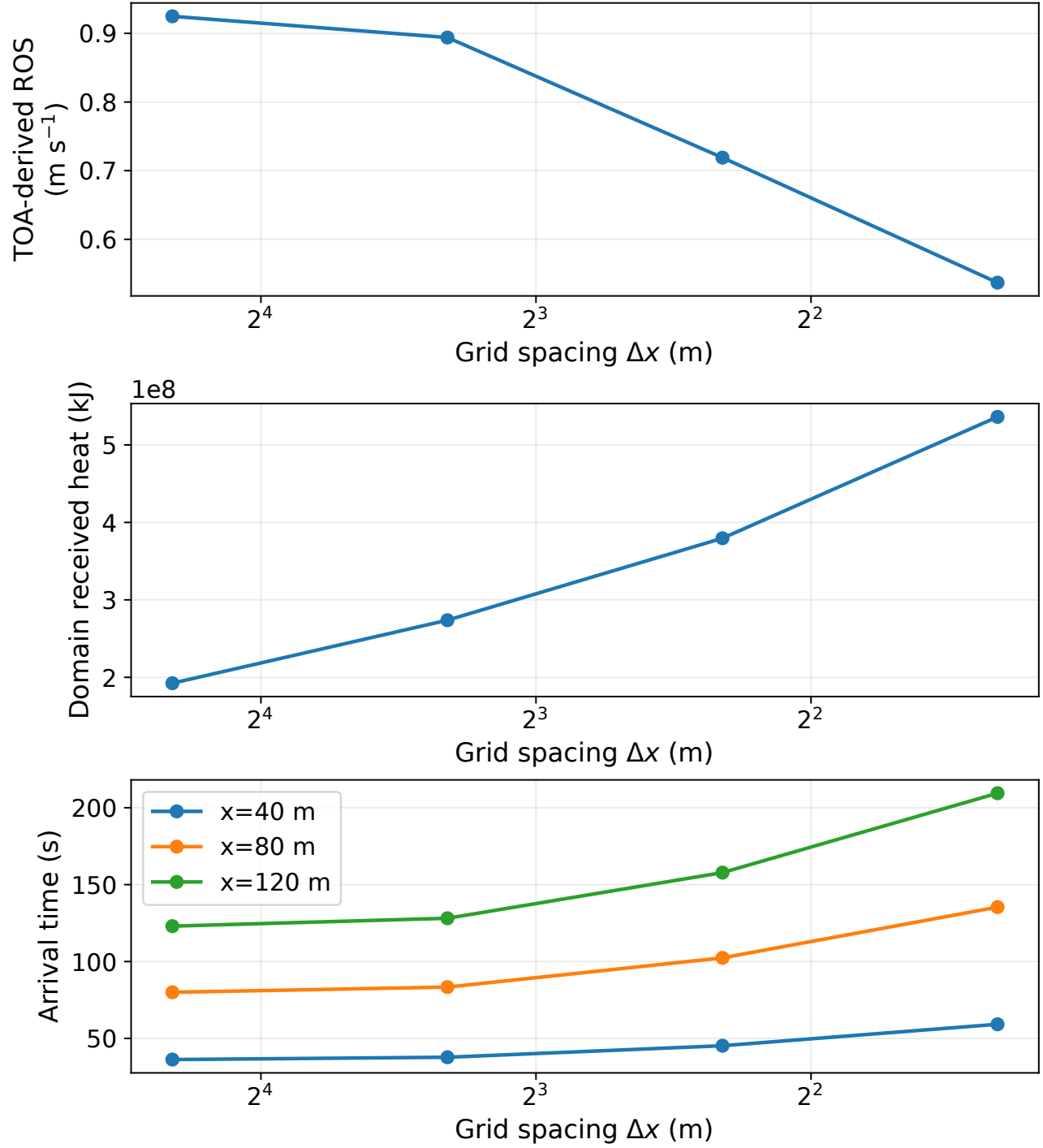
Figure 2: Exact- t = 300 s observables from completed, input-matched simulations; the finest-pair limits are 5% for TOA/ROS and 10% for heat.
