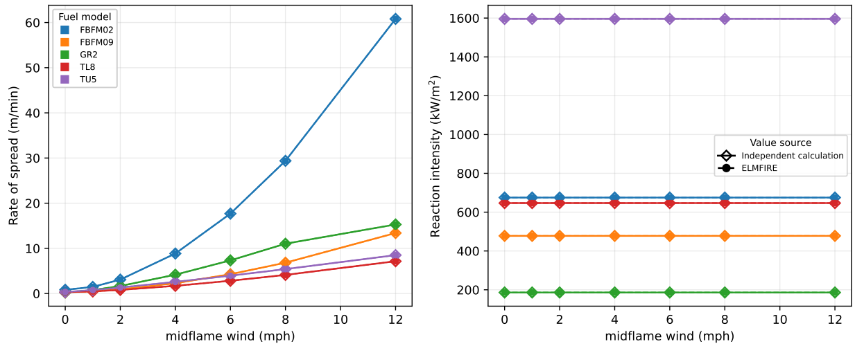
Figure 2: Independent calculations (open diamonds, solid lines) and ELMFIRE predictions (filled circles, dashed lines). Each fuel-model pair uses the same color. Target values are midflame wind; namelists contain the corresponding 20-ft wind.
