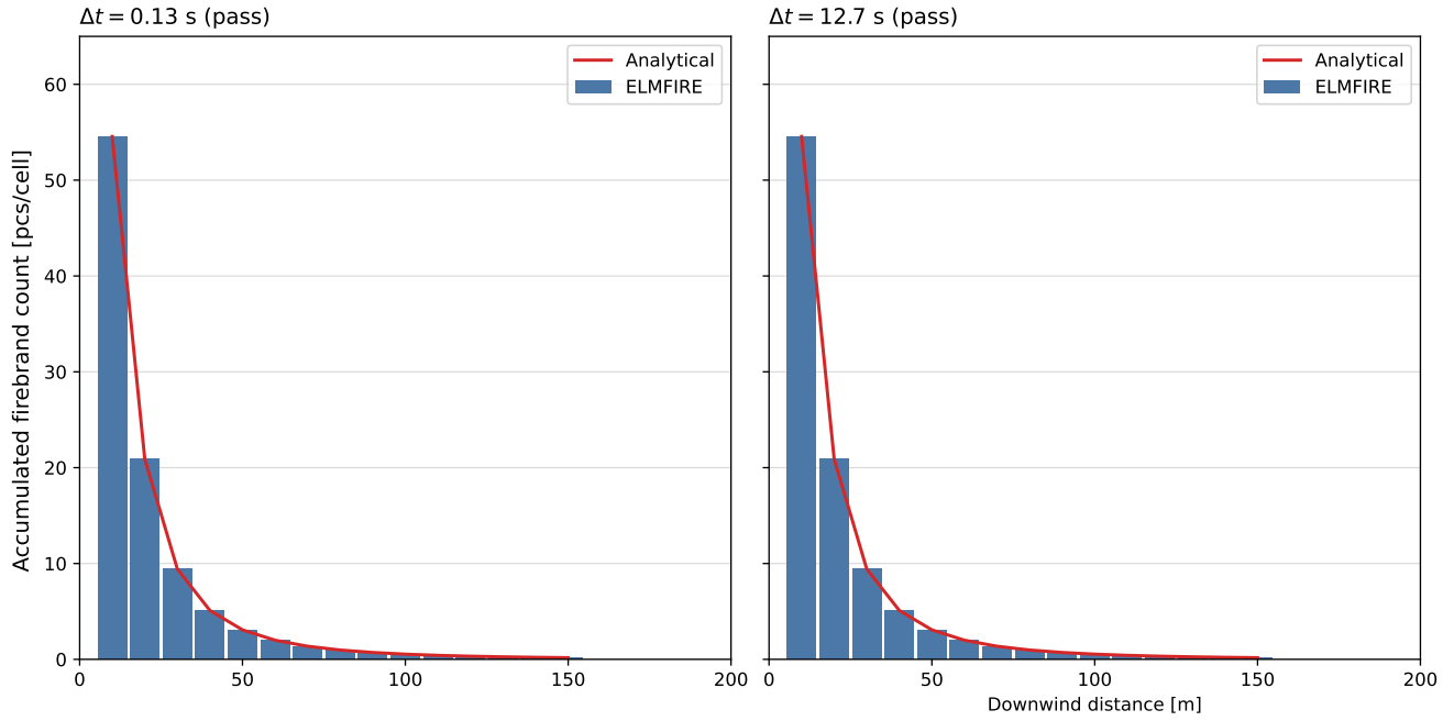
Figure 3: Accumulated firebrands per downwind cell for the 0.13 and 12.7 s timestep simulation conditions. Blue bars are ELMFIRE output and the red curve is the cell-integrated, truncated-lognormal reference for 100 generated firebrands.
