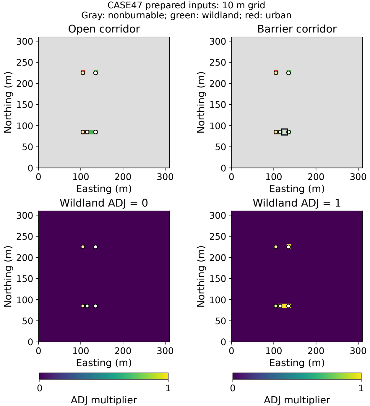
Figure 1: Whole-domain prepared inputs for representative high-HRR simulation conditions. FBFM91 marks each urban source, FBFM1 marks wildland receivers/path cells, FBFM99 is nonburnable, and the black contour is the generated initial PHI interface. Yellow circles mark urban sources; white circles mark wildland receivers. The upper row of markers is the isolated heat experiment; the lower row is the surface-spread experiment, with a square marking the barrier cell.
