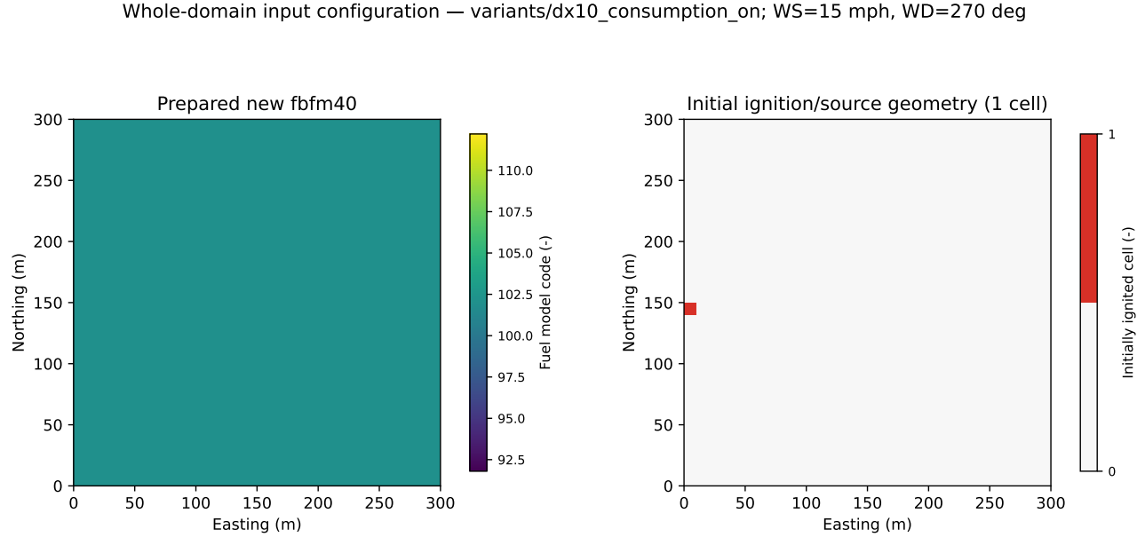
Figure 1: Whole-domain prepared input configuration for the representative simulation condition. The physical domain is shown without the numerical halo; coordinates, configured wind values, fuel or structure layout, and initial ignition/source geometry are identified in the panels.
