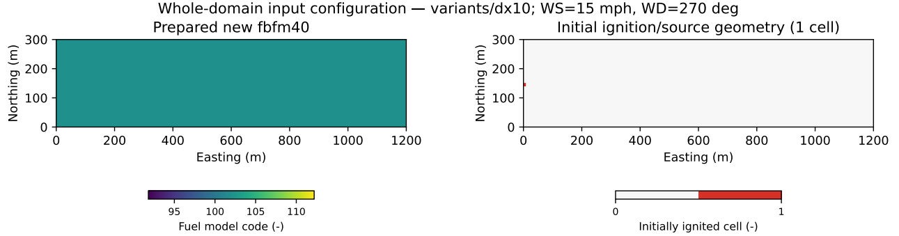
Figure 1: Whole-domain prepared input configuration for the representative simulation condition. The physical domain is shown without the numerical halo; coordinates, configured wind values, fuel or structure layout, and initial ignition/source geometry are identified in the panels.
