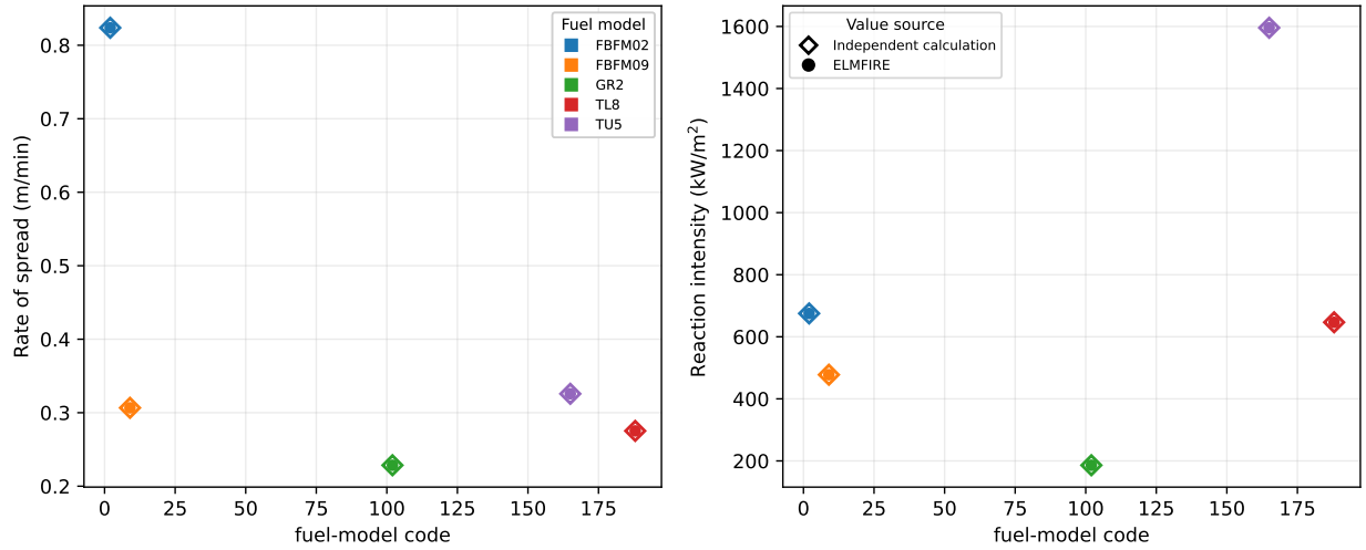
Figure 2: Independently calculated and ELMFIRE rate of spread (ROS, m/min) and reaction intensity (kW/m 2 ) for all five completed standard-fuel simulation conditions. Each fuel model uses one color in both panels; open diamonds denote the independent hand calculation and filled circles denote ELMFIRE.
