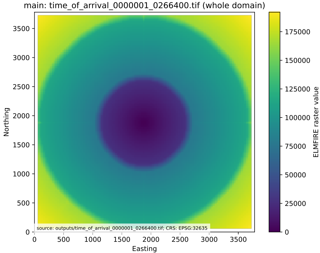
Figure 2: Final whole-domain time of arrival, in seconds, when a case-specific result figure has been generated. The figure must identify its selected GeoTIFF and simulation condition; the generated metrics table, not visual appearance, determines acceptance.
