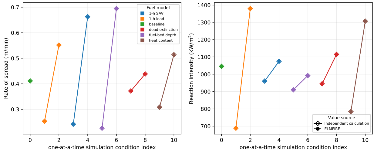
Figure 2: Independent calculations (open diamonds, solid lines) and ELMFIRE predictions (filled circles, dashed lines) for the custom fuel-table simulation conditions. Each comparison pair uses the same color.
