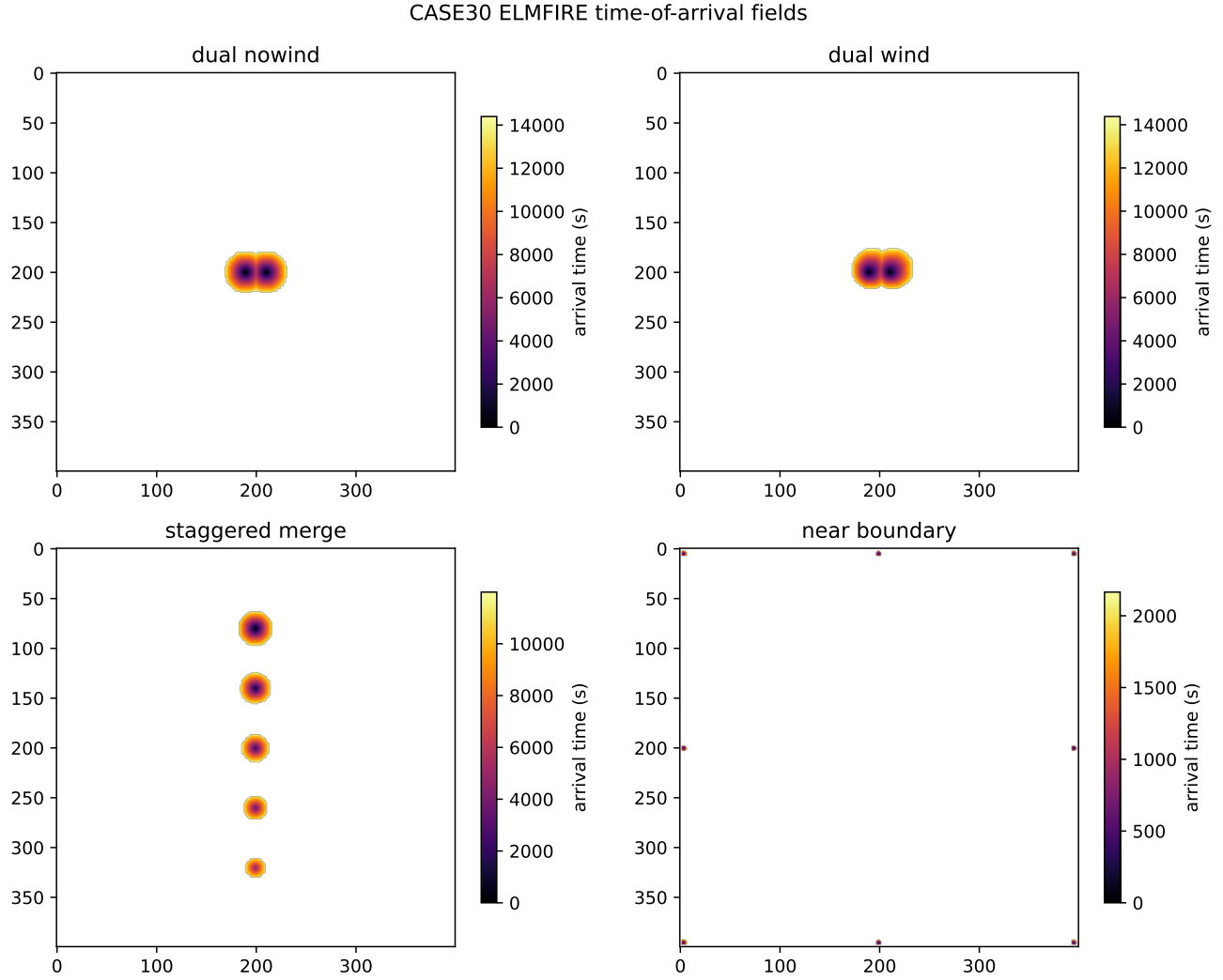
Figure 2: Case-specific time-of-arrival fields for the four ignition-topology simulation conditions.
