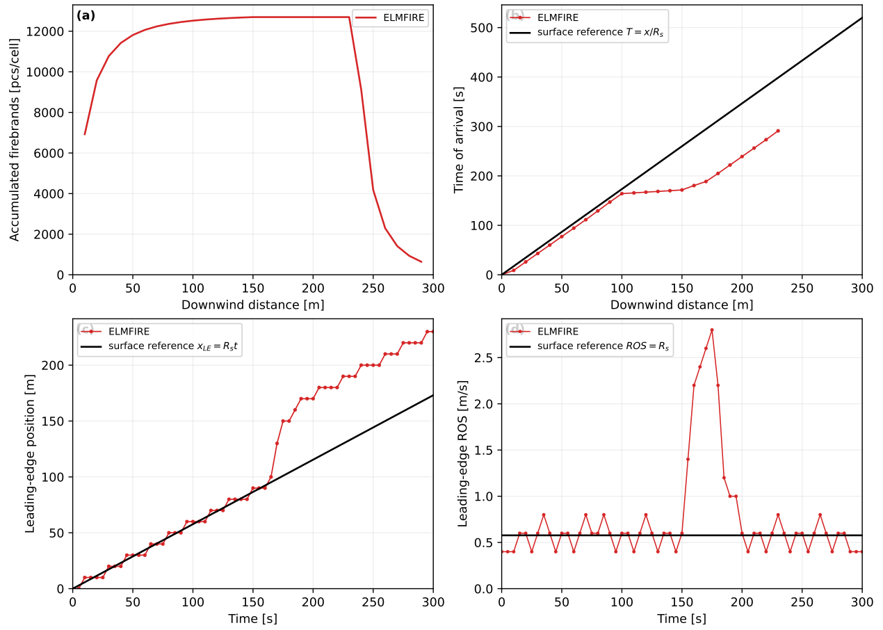
Figure 4: Finite-delay mixed-mode simulation condition. Departure from the surface-only arrival, trajectory, and ROS references identifies firebrand-induced advance.
