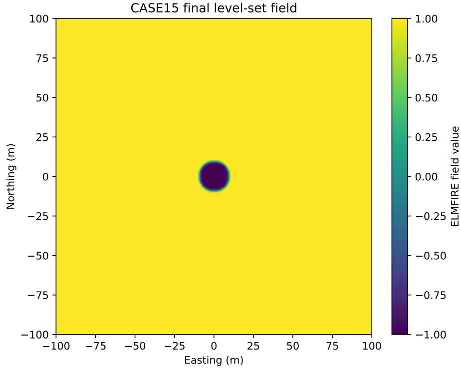
Figure 2: Final whole-domain signed level-set field for the completed simulation condition at the final output time, selected from the results of that simulation condition. Values are dimensionless signed-level-set values; the generated table supplies the acceptance limits.
