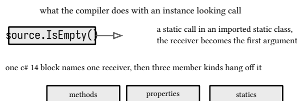
figure 29: extension members, an instance call rewritten to a static one
