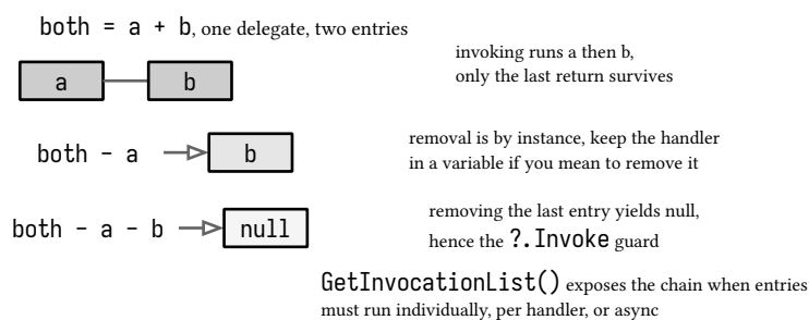
figure 48: the multicast chain, combine, invoke in order, remove by instance
