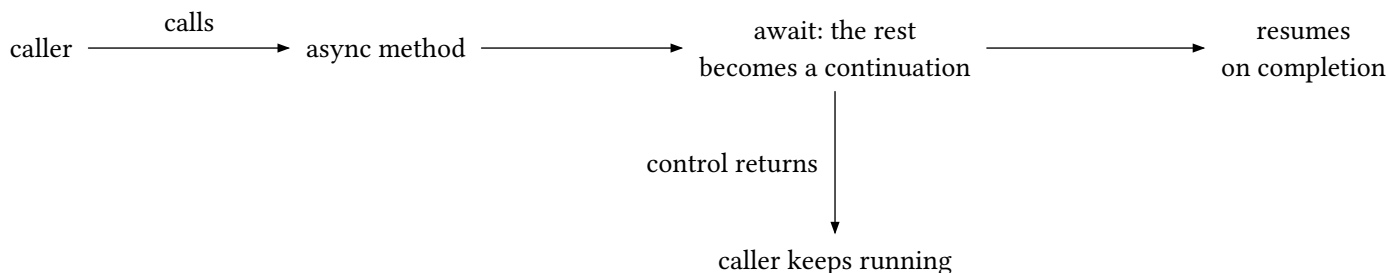
figure 57: await as suspension, one method lowered to a state machine
