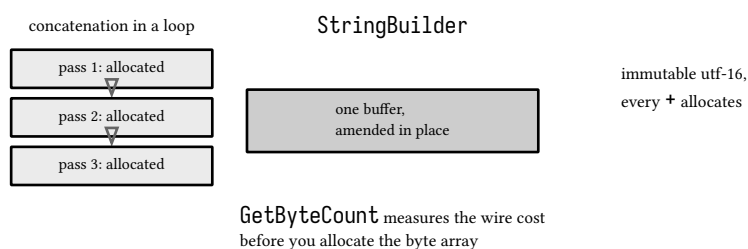
figure 103: string churn against one builder buffer
