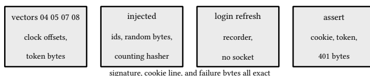
figure 156: an auth golden test: fixed inputs in, frozen bytes out
