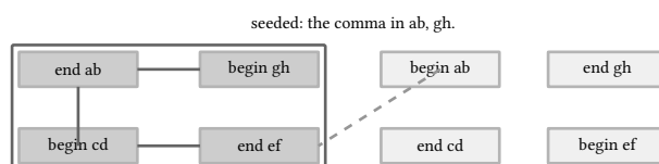
figure 101: the fixture's closure graph: the seeded end(ab) reaches three more vertices, and those four marks are exactly the printed commas
