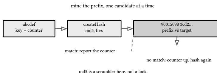
figure 54: the mining loop, hash the candidate, compare the leading hex
