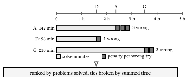
figure 1: how the scoreboard sees one team: solve minutes on the clock plus a penalty block per wrong submission, summed over the solved problems
