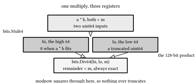
figure 33: the 128-bit product split into halves, divided back to a remainder
