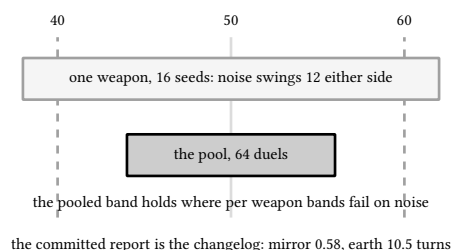
figure 90: the pooled band against the per weapon noise swing
