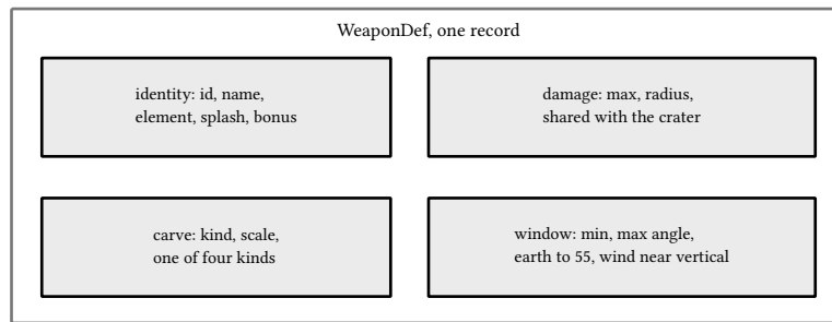
figure 36: the weapon record: identity, two profiles, and a fire window
