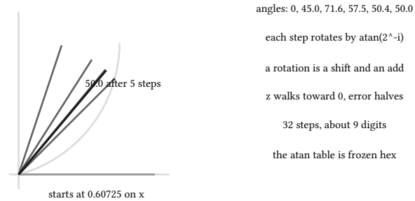
figure 17: cordic walking the vector onto the target angle, one shift-add per step
