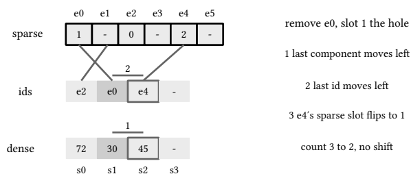
figure 7: the store as three arrays, and a removal paid in three writes
