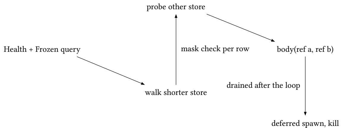
figure 8: a two component query walking the shorter store
