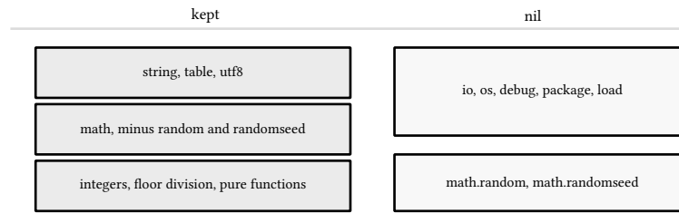
figure 53: what the script sees: arithmetic and tables, nothing that touches the world
