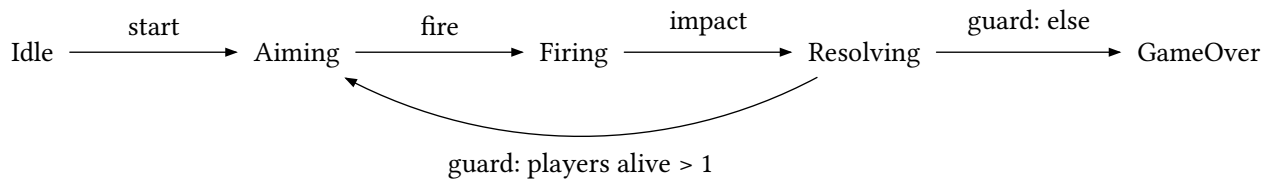
figure 12: the turn machine, one row per arrow
