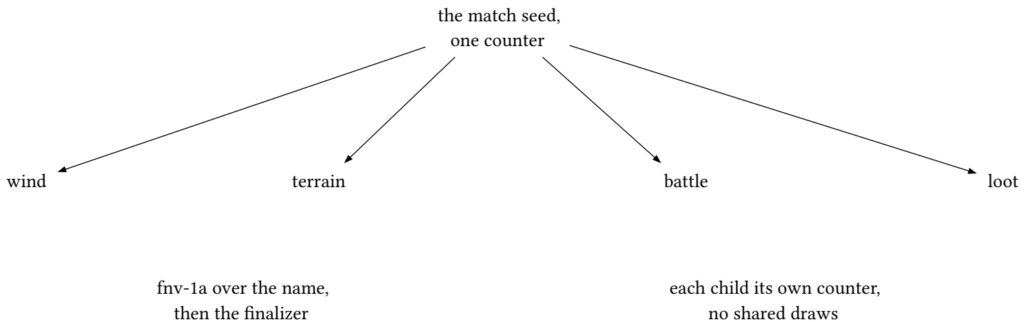
figure 27: the match seed forking named streams, children never share draws
