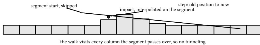
figure 21: one flight step against the heightfield, the crossing column wins
