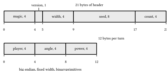
figure 28: the replay file as one byte map, 21 of header, 12 per turn
