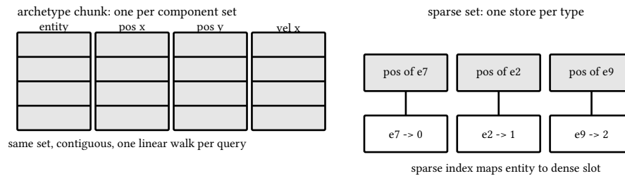
figure 6: the two storage religions, archetype chunk versus sparse set
