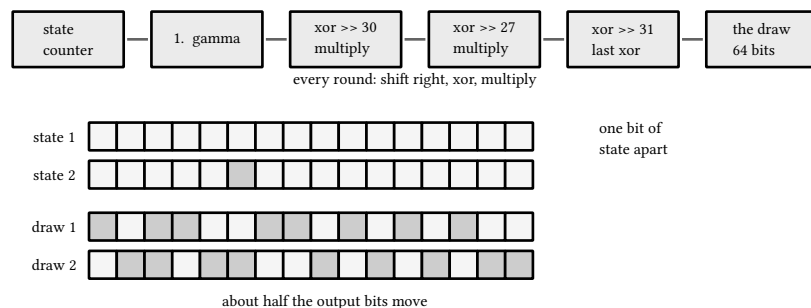
figure 25: splitmix64: a counter through two xorshift-multiply rounds and a final xor
