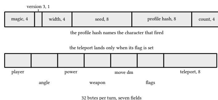
figure 67: replay v3: 29 of header, the profile hash beside the seed, 32 per turn
