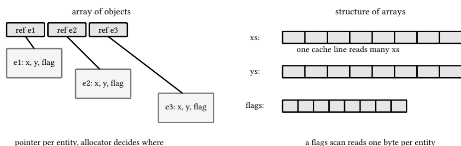
figure 9: the two shapes, array of objects versus structure of arrays
