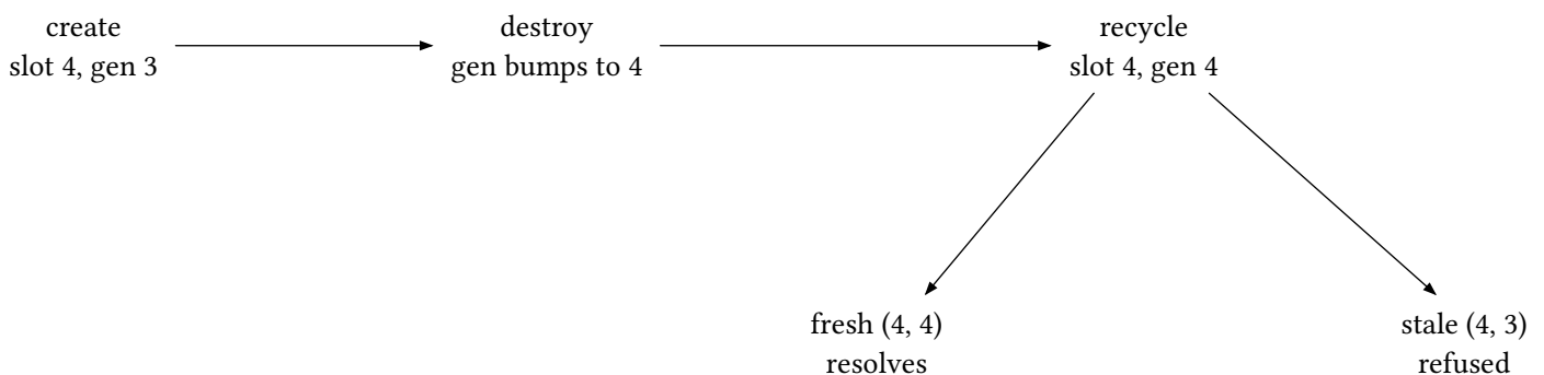
figure 4: one slot's life, and the stale handle refused on use
