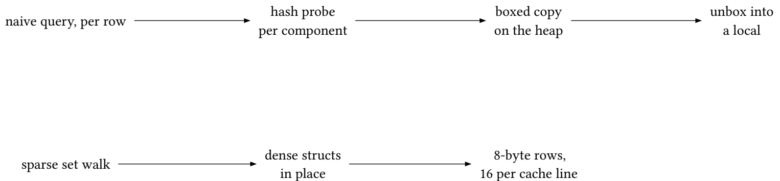
figure 5: one query row: dictionary probes and boxed copies against the contiguous walk
