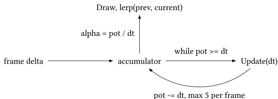
figure 2: the accumulator in one picture
