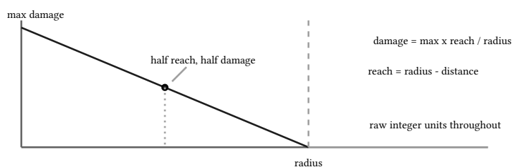
figure 37: linear falloff, full at the impact, exactly zero at the radius
