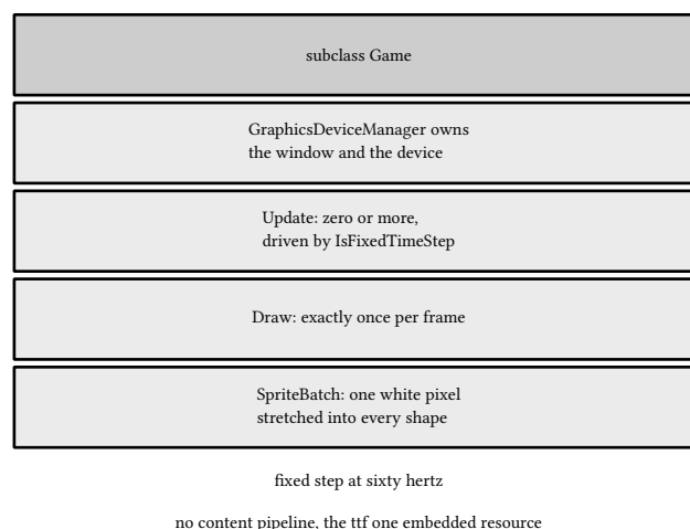
figure 68: the kni Game contract stacked, who owns what each frame
