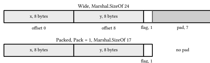
figure 11: wide at twenty four bytes against packed at seventeen, the pad labeled
