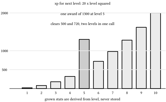
figure 33: the quadratic xp curve, one award crossing two levels
