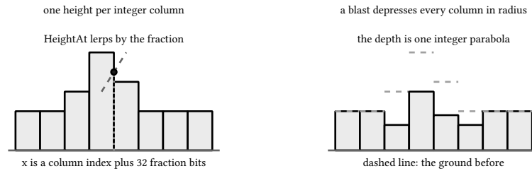
figure 20: the heightfield: lerp between columns, carve an integer parabola
