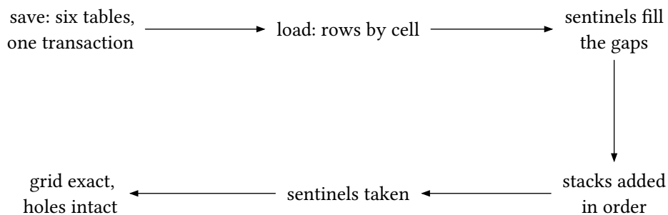
figure 29: the save as one transaction, the grid rebuilt through add and take
