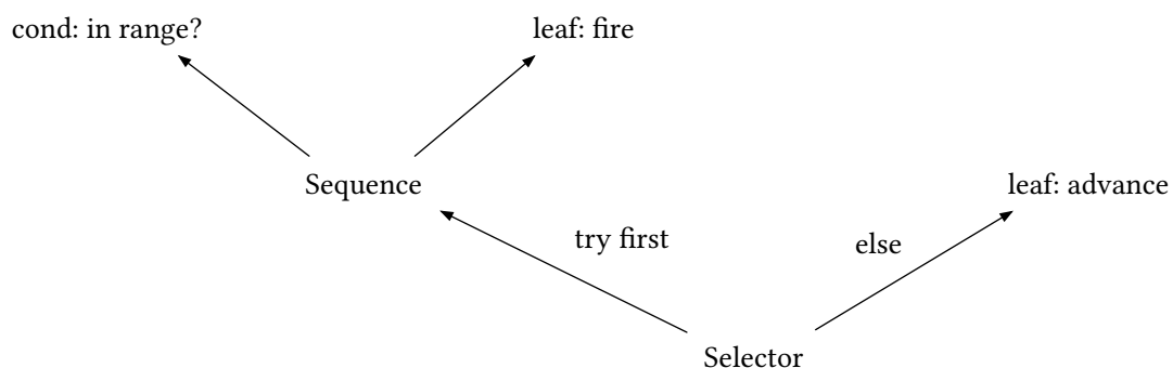
figure 13: the chapter's tree, selector takes the first succeeding child, sequence needs all
