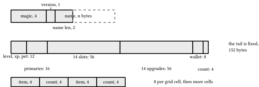
figure 35: the v2 sheet as bytes, name prefix, fixed tail, eight per cell
