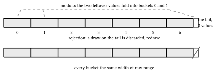
figure 26: seven buckets: modulo folds the leftover, rejection discards it
