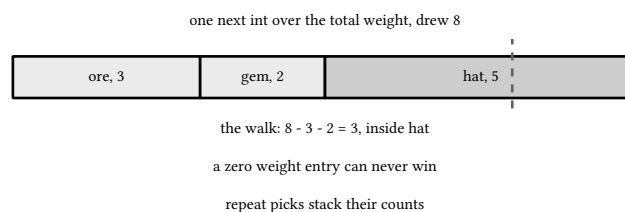
figure 49: one draw over the total weight, the subtracting walk picks
