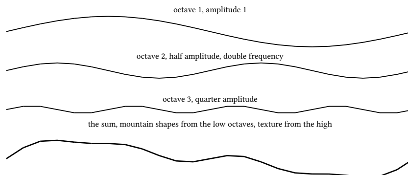
figure 23: octaves at halving amplitude and doubling frequency, and their sum
