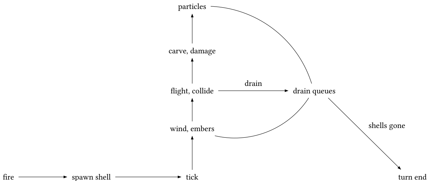
figure 60: one turn through the battle engine's systems
