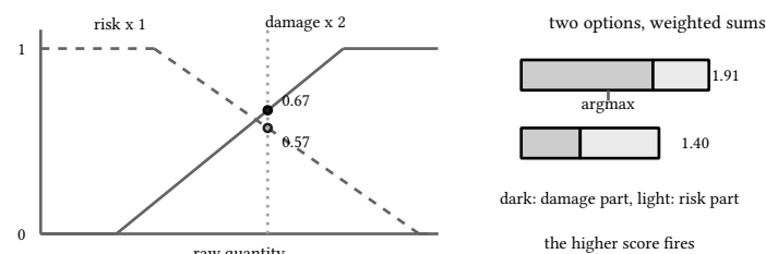
figure 15: response curves onto 0 to 1, weighted sums, argmax picks
