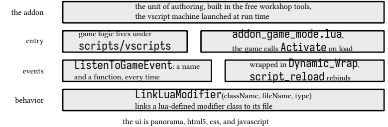
figure 56: dota 2 vscrip: the addon’s entry point, its event listeners, the linked modifier classes
