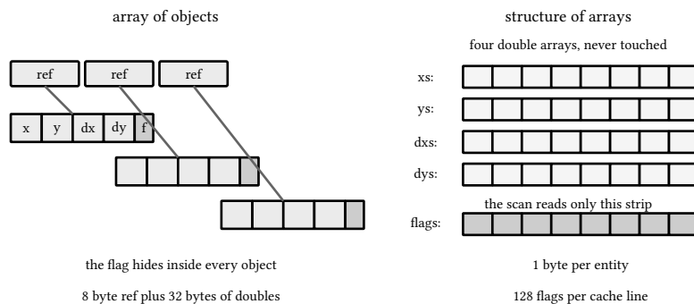
figure 10: which entities are flagged, the bytes each shape must touch
