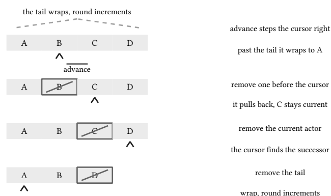
figure 24: one round on the queue, the cursor through advance and three removals
