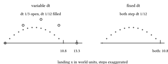
figure 1: the same shot under two step sizes lands apart, the fixed grid lands on one point
