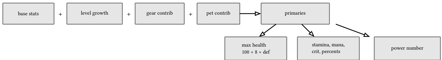
figure 34: the composition stack, growth and bonuses fold into the stats the battle reads
