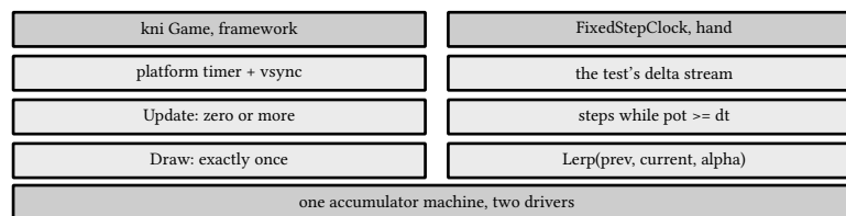
figure 3: the kni game contract stacked against the hand built clock
