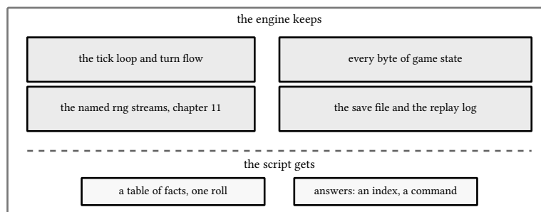
figure 51: the embedding boundary: the engine keeps everything, the script only answers
