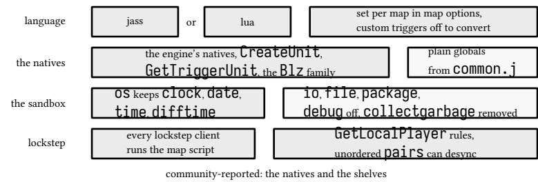
figure 55: warcraft iii: one script language per map, natives as globals, shelves stripped
