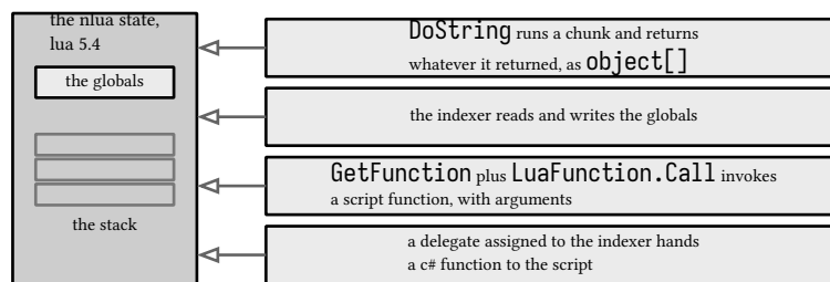
figure 52: the host's four moves over one nlua state, the stack shape the lua book teaches in c
