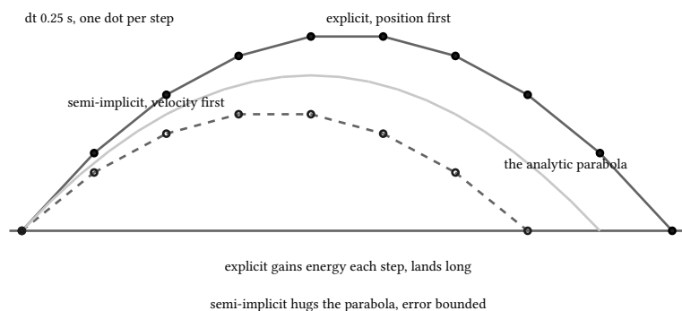
figure 19: one shot, two integrators, explicit gains energy every step
