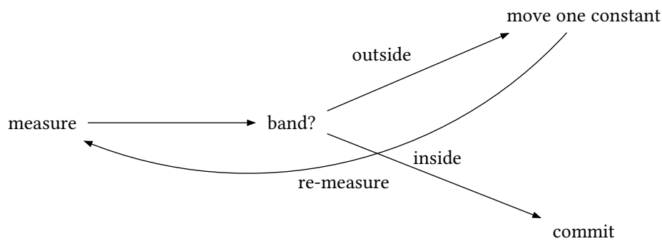
figure 89: the tuning loop, one constant moves per lap
