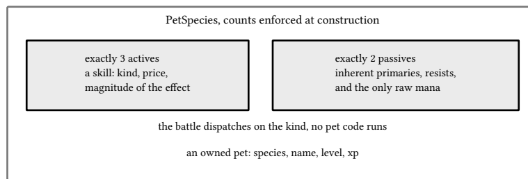
figure 43: the species pinned at three actives and two passives
