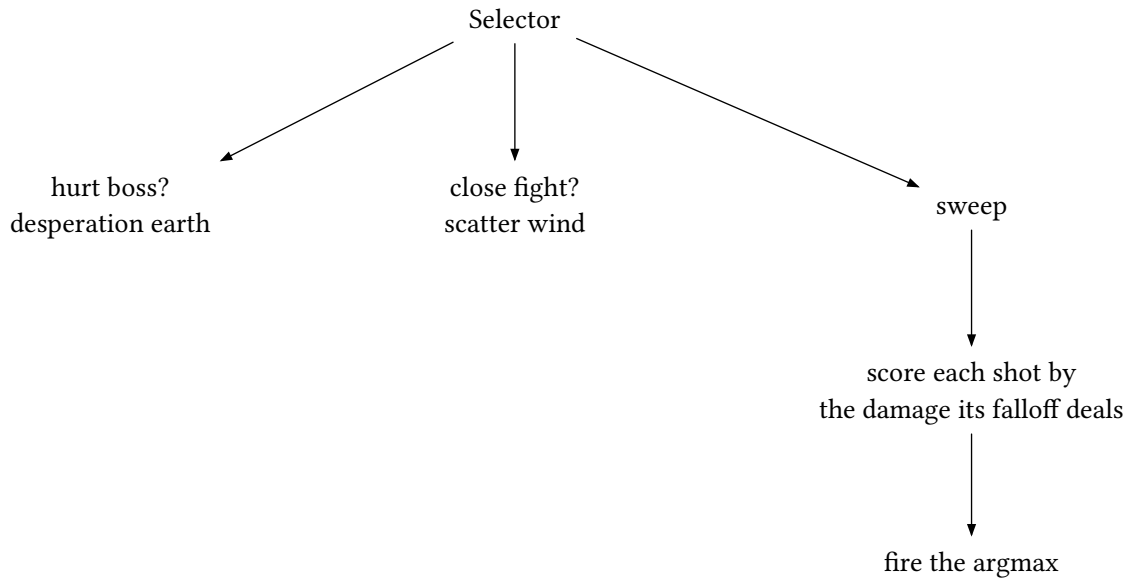
figure 62: the hybrid: a selector over desperation, scatter, and the sweep leaf
