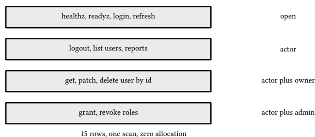
figure 156: the table: rows of routes, flags of requirements, one scan
