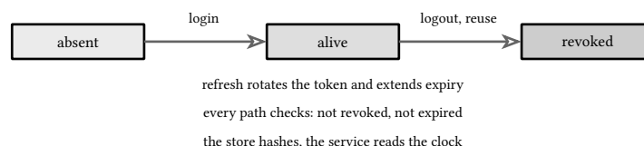
figure 159: the session lifecycle: login creates, refresh extends, logout or reuse revokes
