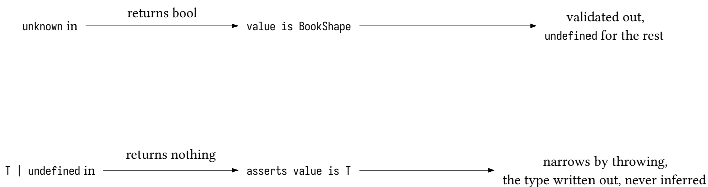
figure 86: two boundary functions, predicate against assertion
