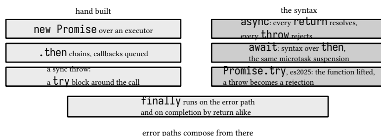
figure 31: the syntax against the hand built forms it replaces
