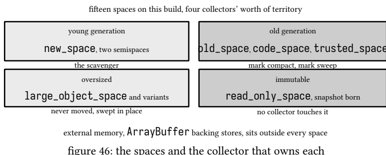
figure 46: the spaces and the collector that owns each
