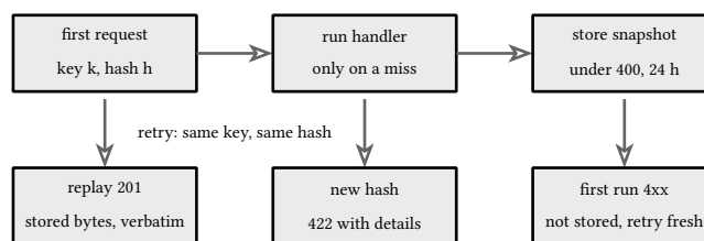
figure 175: one key's life: first run, snapshot, replay, refusal
