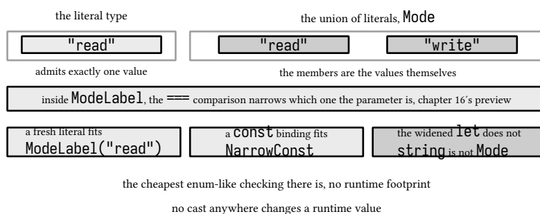
figure 67: literal and union literal types, the members are the values themselves
