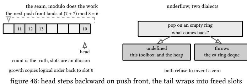
figure 48: head steps backward on push front, the tail wraps into freed slots
