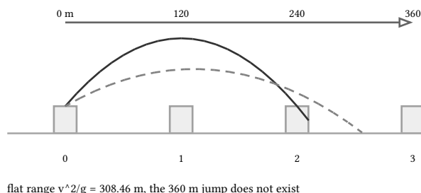
figure 106: cross-section of the flat fixture: the 240 m parabola exists, the 360 m attempt falls to the ground at the 308.46 m range limit
