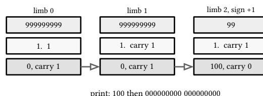
figure 7: the carry chain across all three limbs: each full base records a zero limb and passes one up, the top limb absorbs the last
