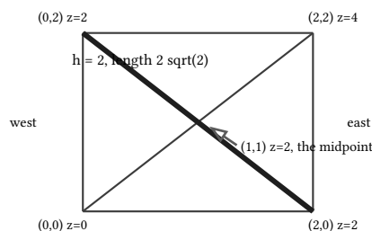
figure 174: the two triangles in plan view, elevations at the corners, and the level-2 polyline through (2,0), (1,1), (0,2) bolded
