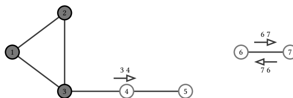
figure 123: the fixture graph: the triangle core keeps the sign at its boundary street, the two peeled vertices render hollow, and the isolated tree keeps both leaf signs
