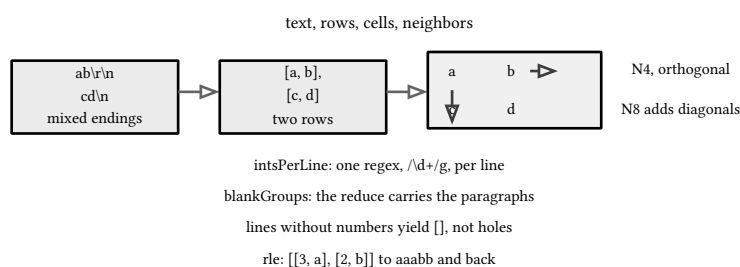
figure 52: text to rows to cells, the deltas ready for the walk
