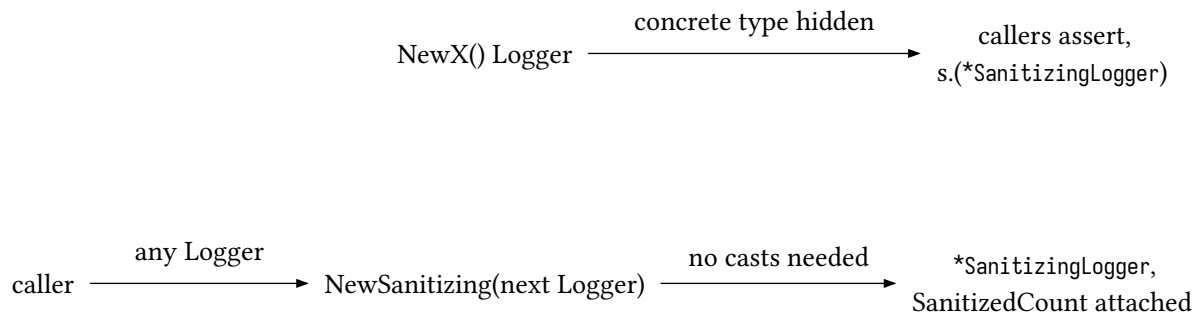
figure 2: any logger in, the concrete sanitizer out, the reverse hides the type
