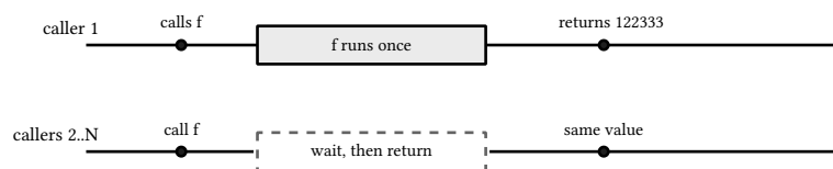
figure 38: one caller runs f , the rest wait and replay the value
