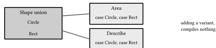
figure 24: one closed union, visitors are switches over it
