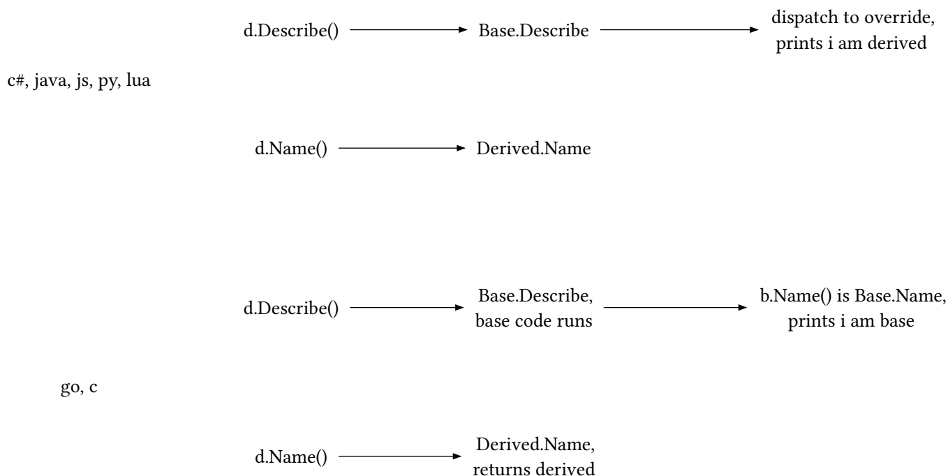
figure 3: go and c forward, the five class-dispatch languages reach the override
