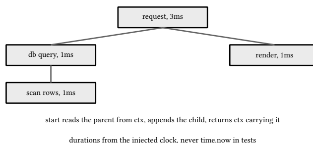
figure 79: the span tree grows through the context, one child per start
