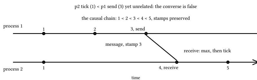
figure 57: local events tick, receive takes the max then ticks, order is one way
