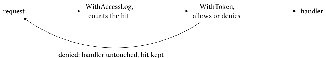
figure 14: the chain folds outside in, a denial is still a counted hit
