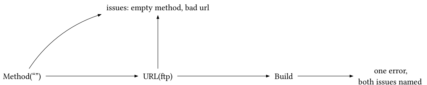
figure 8: issues accumulate across the steps, build joins them into one round trip
