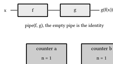
figure 27: pipe reads left to right, a closure is a private cell
