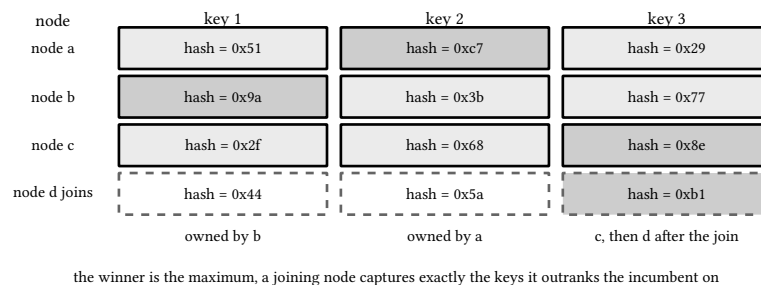
figure 70: highest random weight: per key, every node is scored, the max owns it
